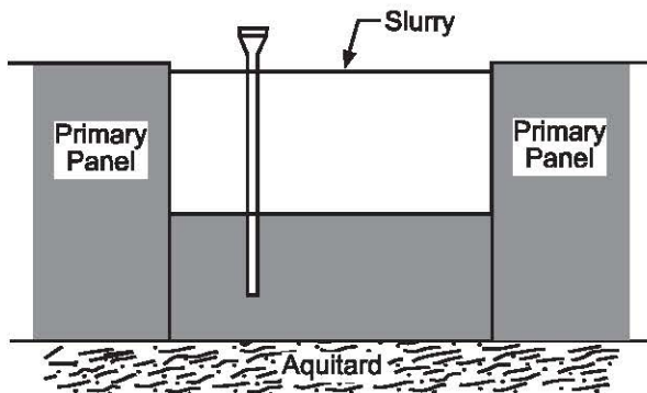
Figure 5(e) Tremie concreting secondary panel
