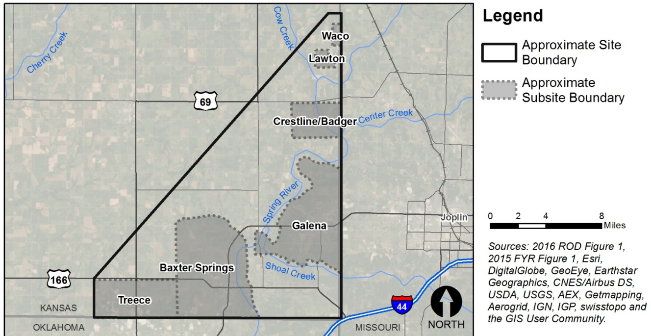
Figure 5. The Cherokee County Superfund site, subsites and surrounding areas.
