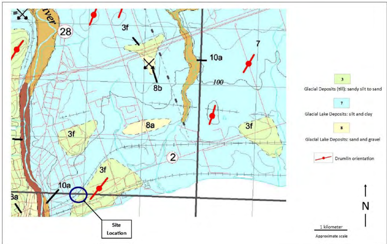
Figure A16. An excerpt from local surficial geology map (Brennard, 1997) showing the site is located on the crest and western side of a drumlin (green area with axis of orientation shown in red) which is surrounded by fine (silts and clays) lake deposits.
