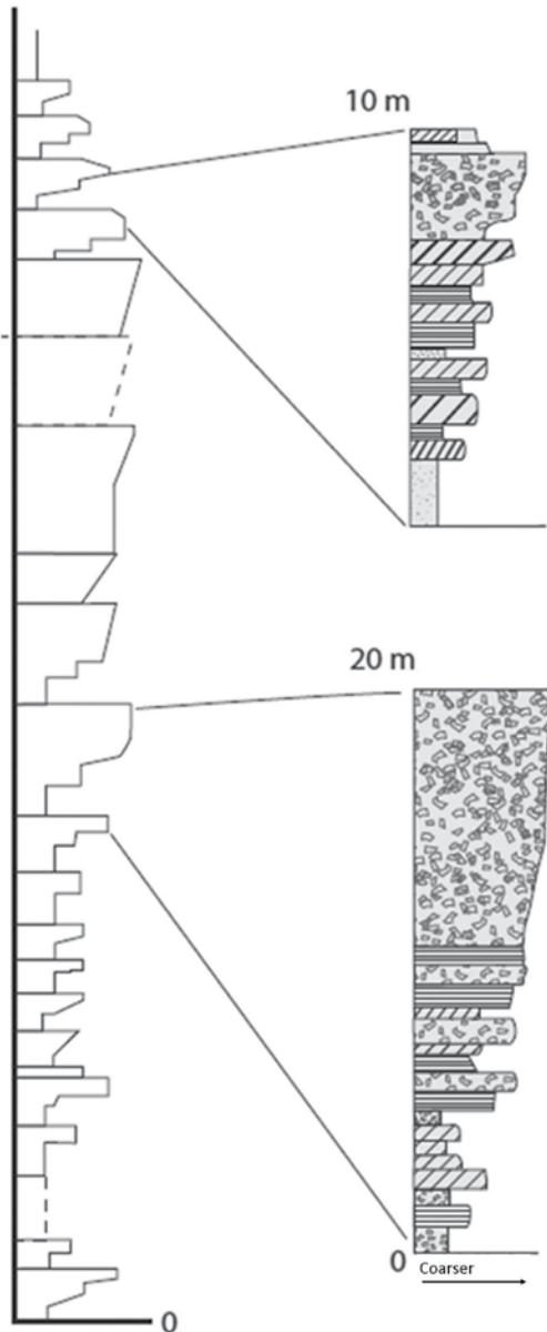
Figure A20. Vertical profile through cyclic alluvial fan deposits, showing the characteristic coarsening-upward profiles of individual packages which stack to form the overall alluvial fan. (Redrawn from Steel and Gloppen, 1980)
