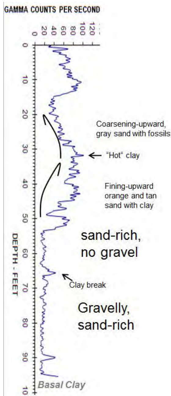
Figure A30. Gamma ray log representing grain size trends and significant clay spikes.
