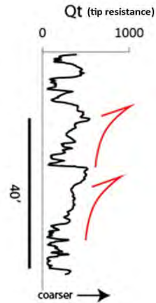
Figure A21. Cone penetrometer testing data show two stacked coarsening-upward sequences (red arrows) separated by thin clay units.
