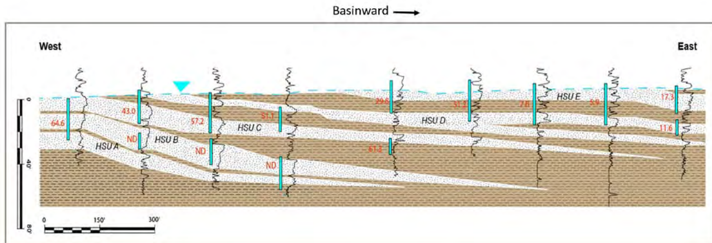
Figure A22. Stratigraphic cross section with CPT logs showing shingled, dipping alluvial fan deposits in the saturated zone.
