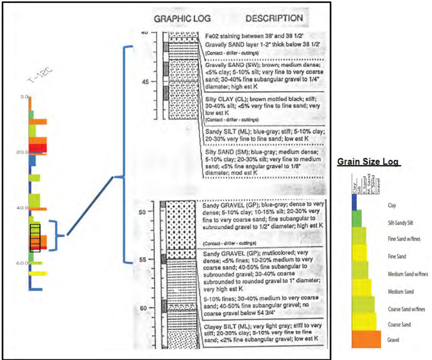
Figure A4. Data formatting for stratigraphic analysis. Portion of a boring log from the site illustrating a clear fining-upward sequence from 55' to 41' bgs representing a channel-fill and abandonment deposit (see Figure A2). Basal gravel lag and overlying fining-upward sequence occurs at 41' below ground surface (bgs). Lithologic contacts were identified on the basis of sampling, cutting returns and drilling behavior. Graphic grain size log (at left) shows this fining-upward sequence within a well screen interval.
