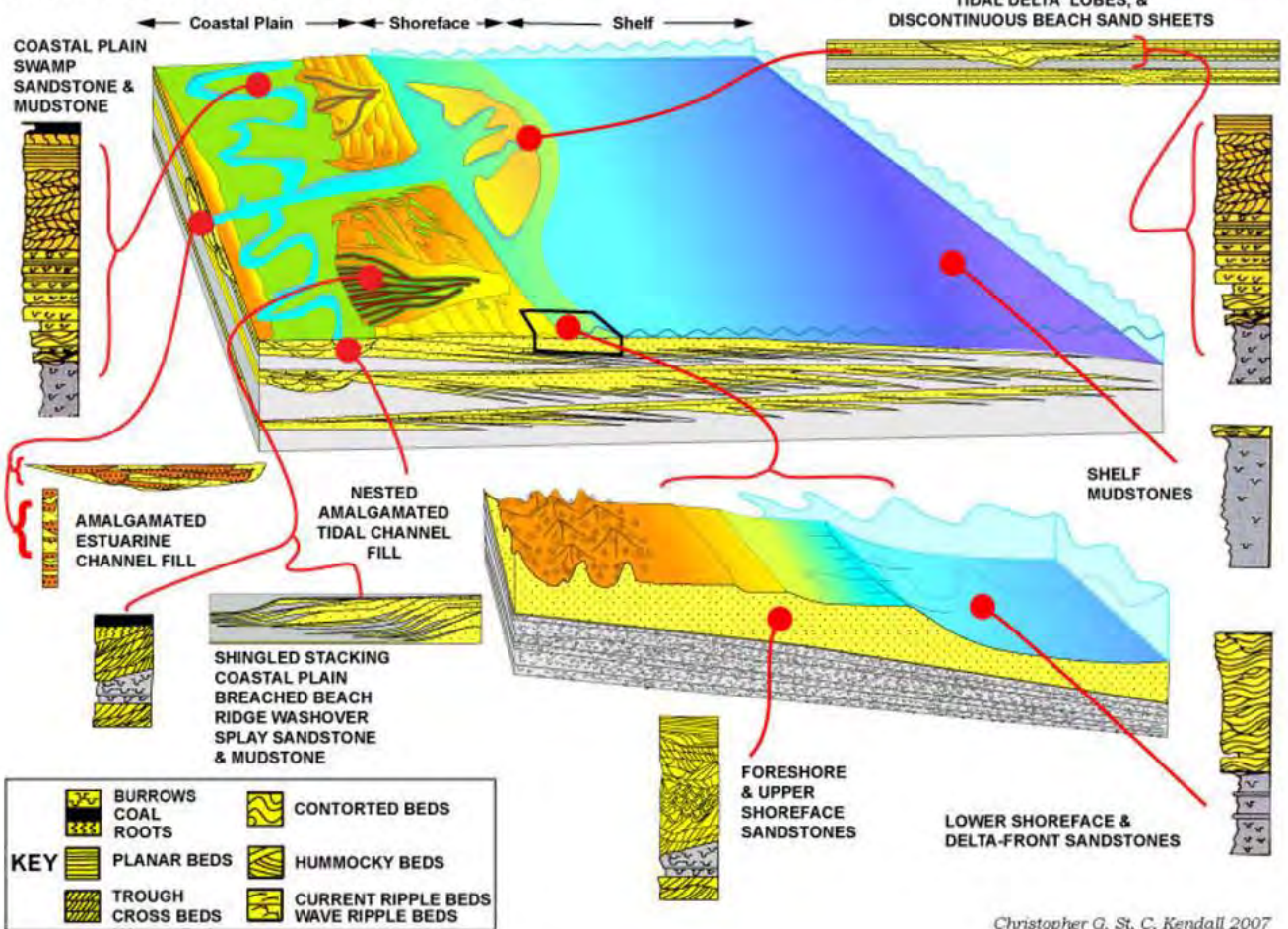
Figure 4. Three dimensional facies model of a prograding barrier shoreline developed through integration of observations of modern barrier island systems, outcropping ancient systems, and subsurface datasets worldwide. “Prograding” refers to the shoreline system migrating seaward, due to an abundance of sediment being supplied, falling sea level, or both (the converse is referred to as “retrograding”). Note the “sheets” of the barrier island beaches, the “lobes” of the ebb tidal deltas, the “stacked and amalgamated channel fill” and “shingling” of the washover splay sandstones. Each sub-environment has corresponding vertical grain size trends. Scale has been intentionally omitted, as a variety of scales exist for each sub environment. This depositional model applies to many remediation sites located in coastal areas of the Atlantic and Gulf Coasts of the United States as well as coastal regions worldwide. From http://www.sepmstrata.org/CMS_Files/553_lecture1_introduction.ppt Used under Creative Commons fair use policy with thanks to Dr. Christopher G. St. C. Kendall.
