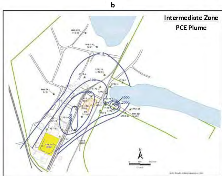
Figure A33. Original CSM (prior to ESS evaluation) is based on the following: A33a shows groundwater elevation contours for the Intermediate Zone with a northeast groundwater flow direction, and A33b shows PCE concentration contours interpreted prior to the lithofacies interpretation and based on this northeast flow direction alone. This interpretation of the contaminant distribution did not take into account the underlying geology. However, as a result of the ESS evaluation, A33c is a lithofacies map of the Intermediate Zone (depicted on this cross section A33d) that shows higher permeability sand channels trend almost perpendicular to the groundwater gradient, bringing to question the chemistry concentration contours interpreted in Figure A33b. Potential action would be to collect groundwater data along the high permeability zones to better define contaminant extent.
