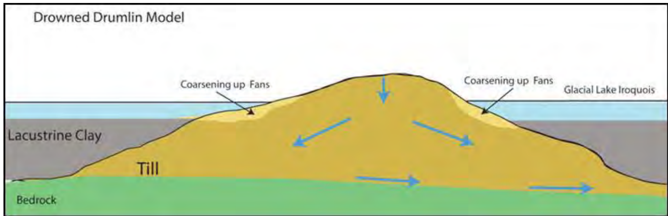
Figure A17. Conceptual summary cross section – Drowned Drumlin Model. Blue arrows are interpreted groundwater flow.
