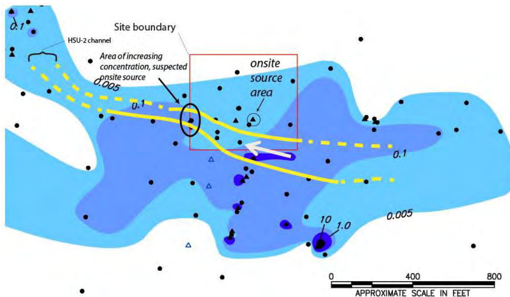
Figure A10. ESS-based CSM focused on underlying geology to define HSUs. The HSU-2 channel (bounded by yellow lines) controls the contaminant migration pathway (white arrow) showing that, unlike Figure A9, an off-site source is contributing to the impact occurring at the property boundary. At this complex site, groundwater flow is strongly influenced by lithology, and contaminant transport directions deviate significantly from those predicted from the potentiometric surface maps.
