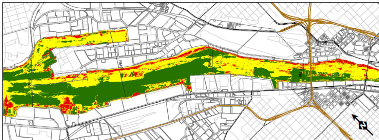
Figure 3.4-20. Sediment Deposition Rates
