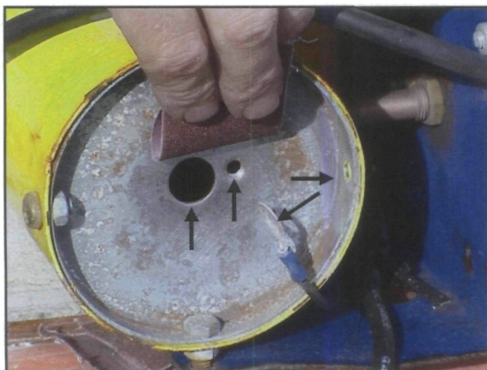
Figure 3. Cleaning points. Use emery cloth or similar material to remove any rust or corrosion from these key points.
