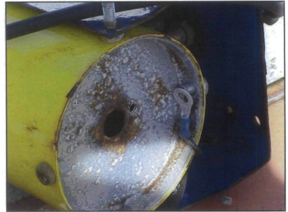
Figure 2. Corrosion of rear cover and ground wire. Remove ground wire from rear cover.
