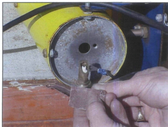
Figure 5. Clean contact points.
