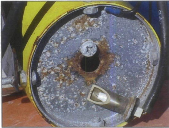
Figure 1. Corrosion of rear cover and electrode. Remove electrode from rear
