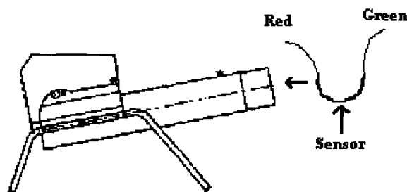
Figure 2. Inserting sensor into cannon barrel
