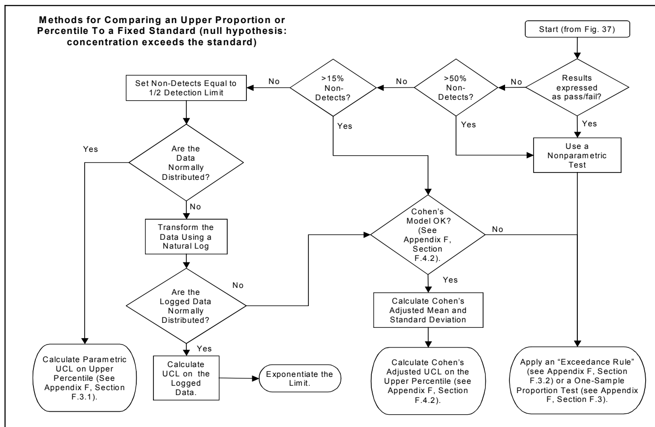
Figure 39. Flowchart of statistical methods for comparing an upper proportion or percentile to a fixed standard (null hypothesis is "concentration exceeds the standard")
