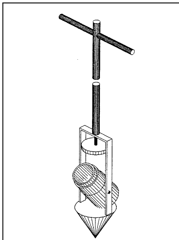
Figure E-10. Lidded sludge/water sampler
