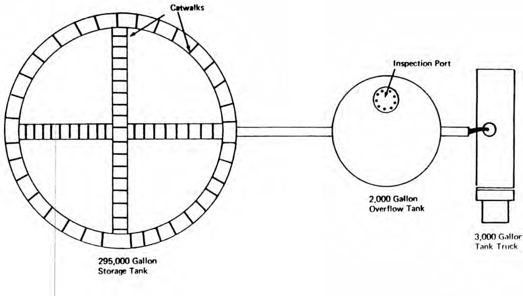
Figure 9-6. Bird's eye view of waste tank, overflow tank, tank truck and connecting plumbing.
