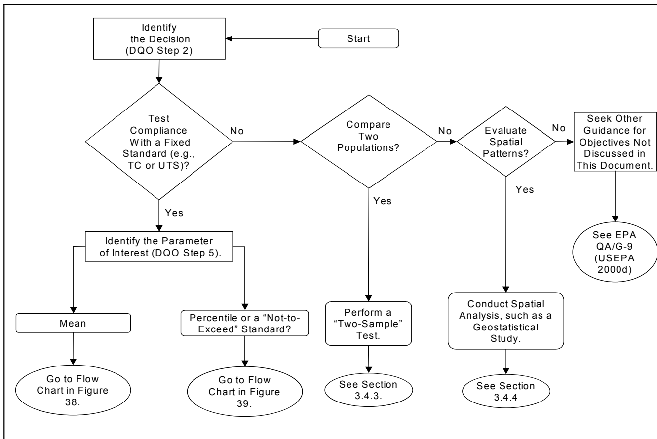
Figure 37. Flow chart for selecting a statistical method
