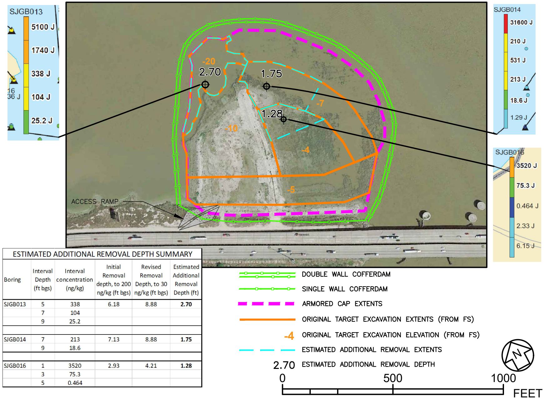
Figure 35 - Selected Remedial Action (Alternative 6N) Cleanup Level: 30 ng/kg
