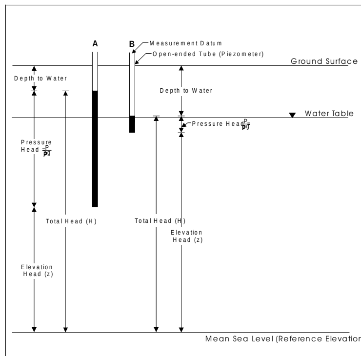
Figure C.3.2 Hydraulic head.
