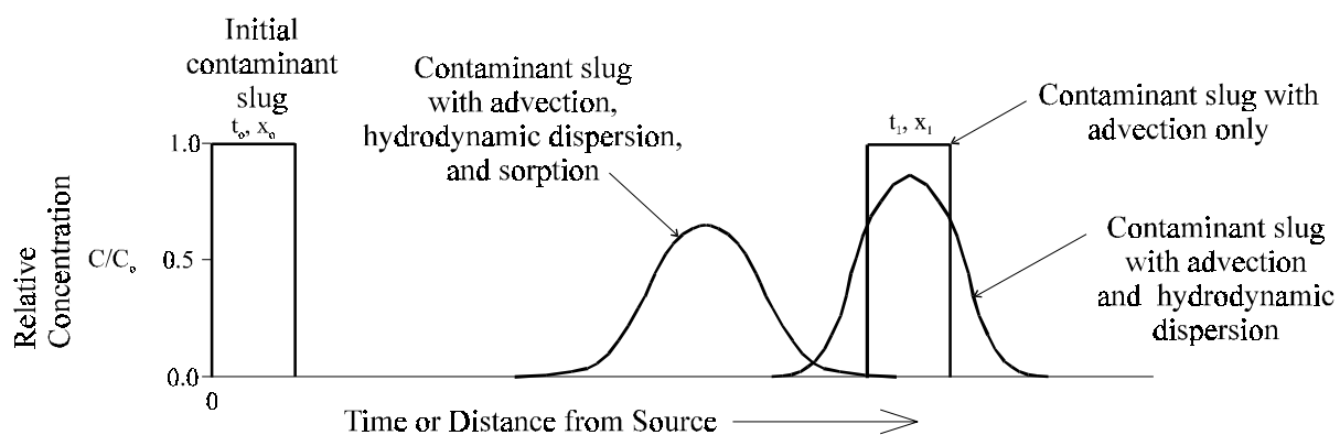
Figure B.2.9 Breakthrough curve in one dimension showing plug flow with instantaneous source resulting from advection only; the combined processes of advection and hydrodynamic dispersion; and the combined processes of advection, hydrodynamic dispersion, and sorption.
