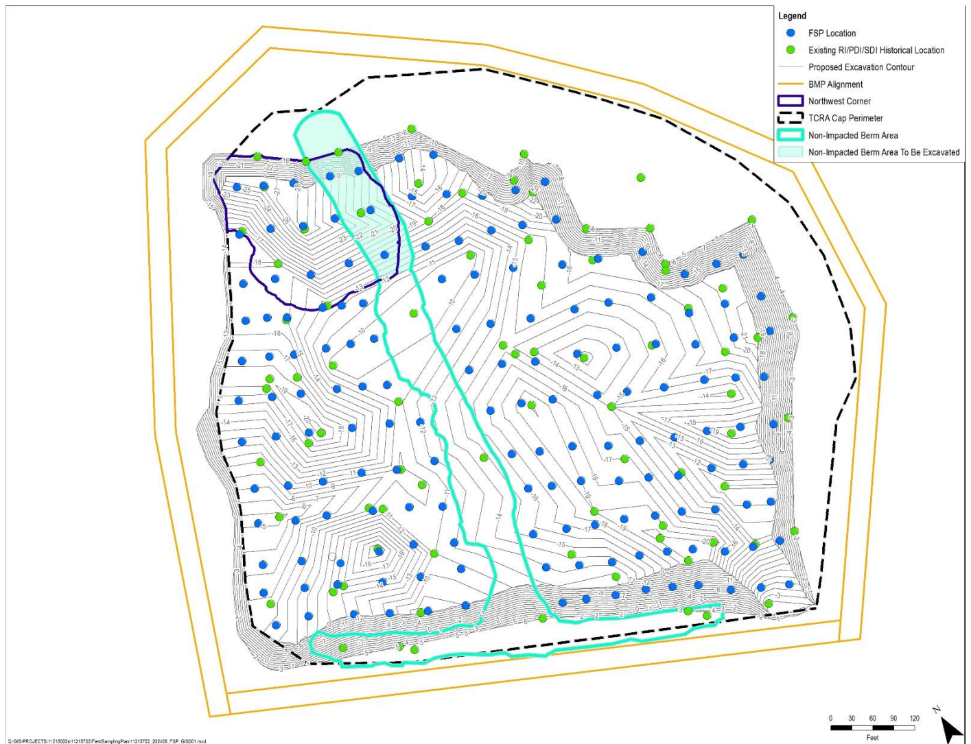
Figure 2.1 Pre-Excavation Sampling Locations with Existing RI/PDI/SDI Locations
