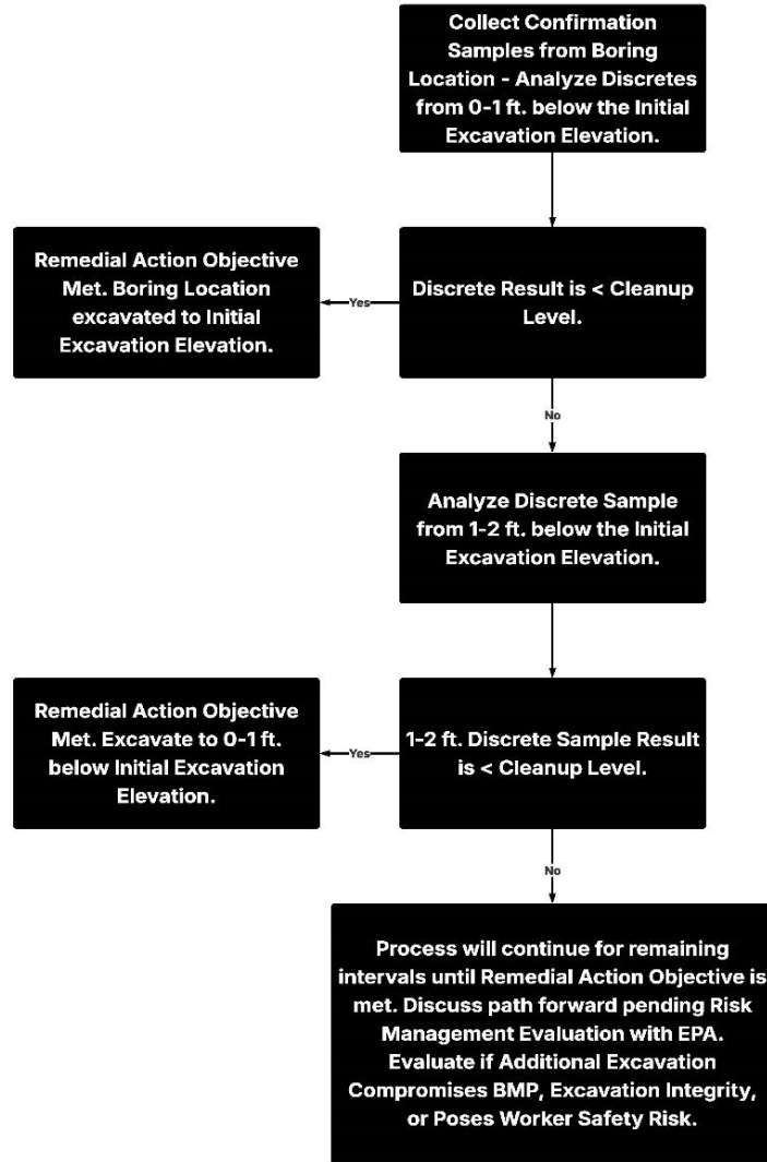
Figure 2.3 Pre-Excavation Sampling Decision Flow Chart
