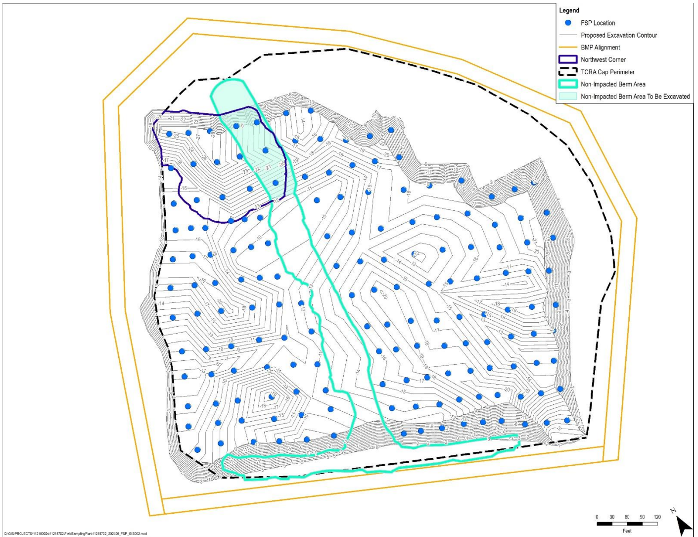
Figure 2.2 Pre-Excavation Sampling Locations
