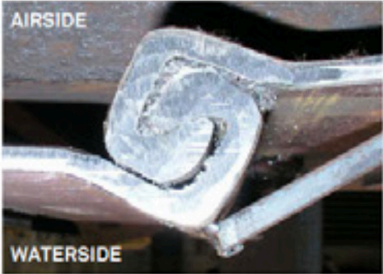
Larssen connectors
