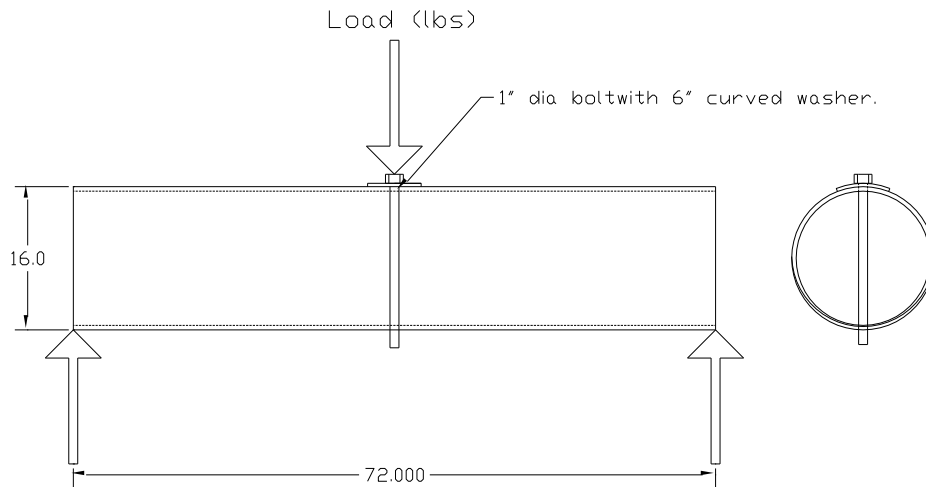
Figure 5: Connection Test B Setup
