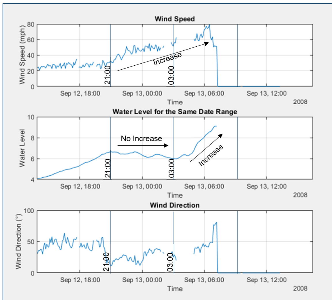
Figure 8 Time Series of Wind and Water on September 12-13, 2008.
