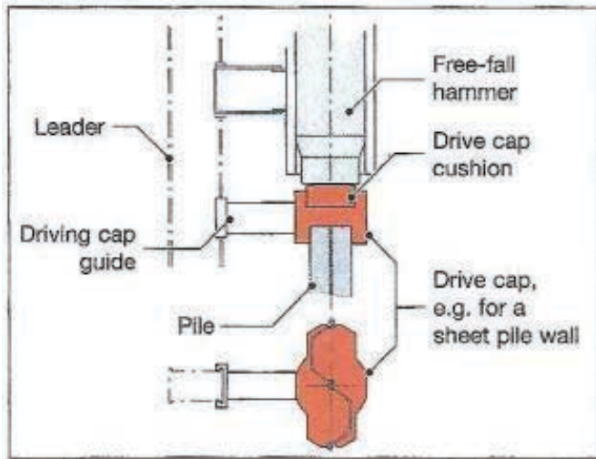
Typical driving cap and spreader plate detail
