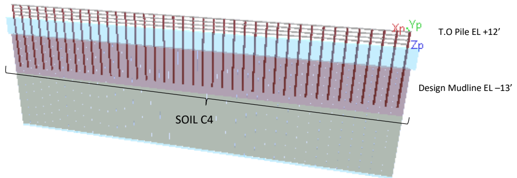
Figure 5: Section 3 Fender Layout - Soil Profile C4
