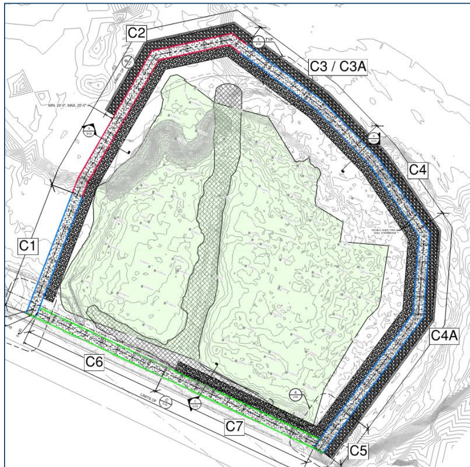
Figure 6.1 General Extents of the Analysis Cross-Sections
