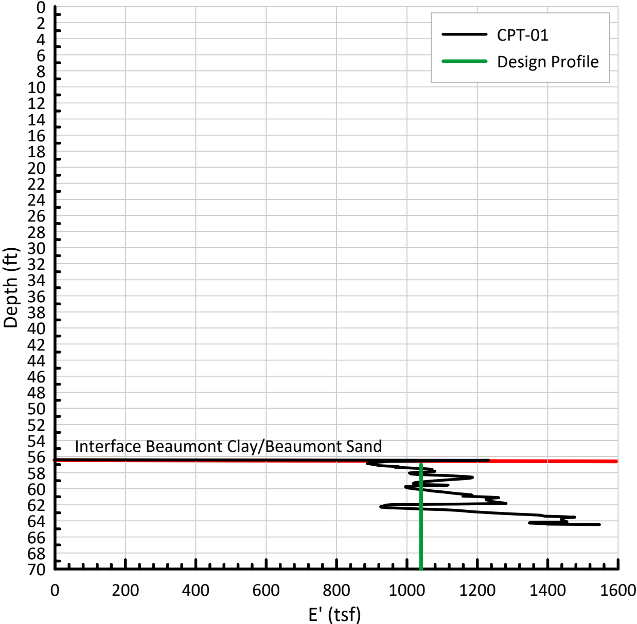
Es - Beaumont Sand - Sectors 1 to 3
