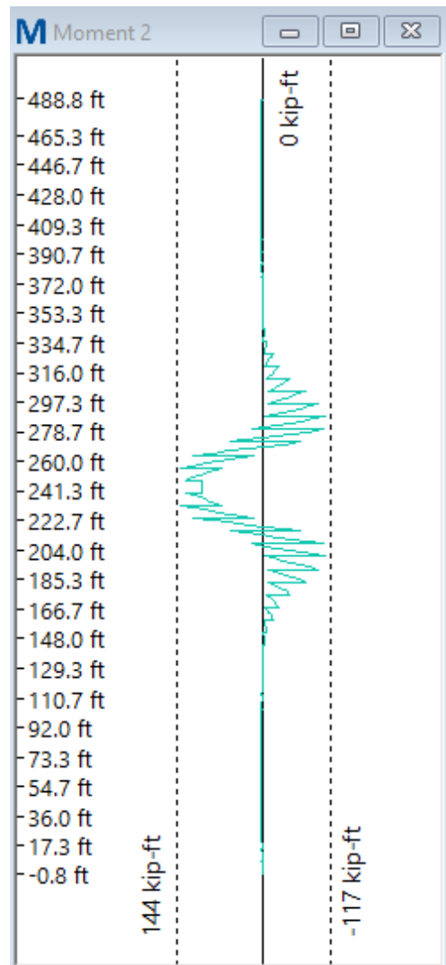
Figure 56: Max Wale Moment - Load Case 5 (Section 4 – Soil C4)
