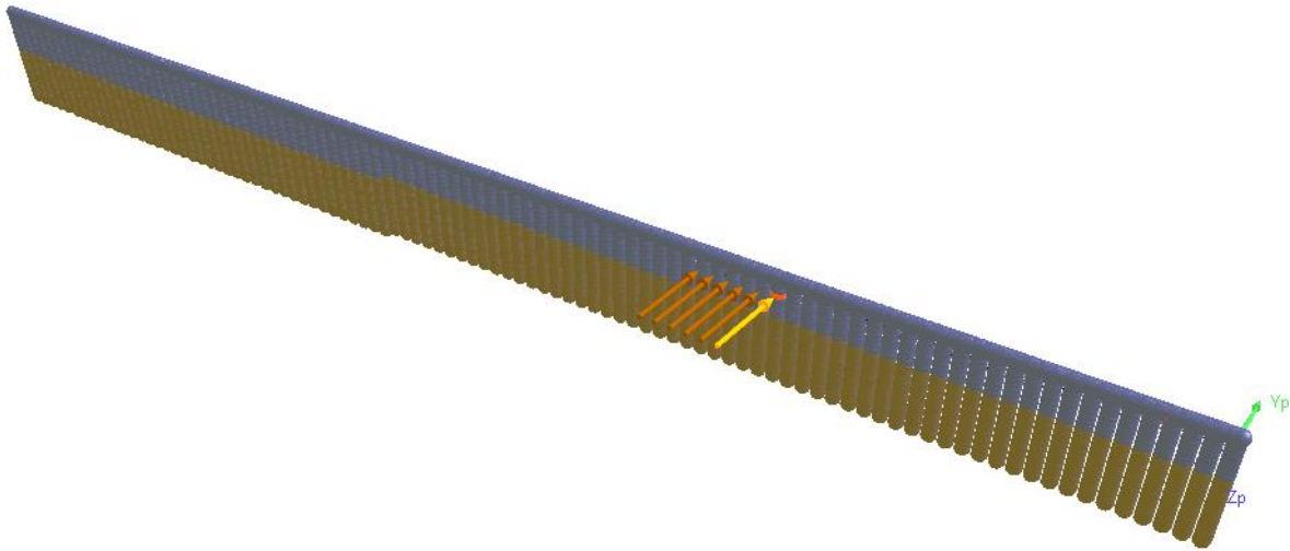
Figure 68: Layout – Load Case 8 (Section 2 – Soil C3)
