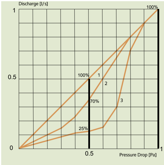
Figure 6.14 Discharge - Pressure Drop Relationship, Arcelor Mittal
