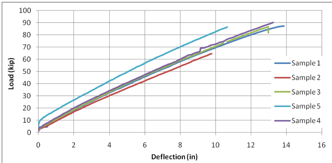
Figure 8: 16 inch Vinyl Ester Four-Point Bend Load-Deflection Response
