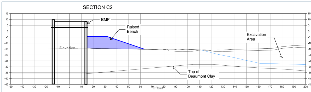
Figure 6.3 Analysis Cross-Section C2
