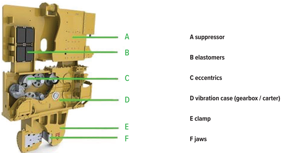
The design of a vibratory hammer
