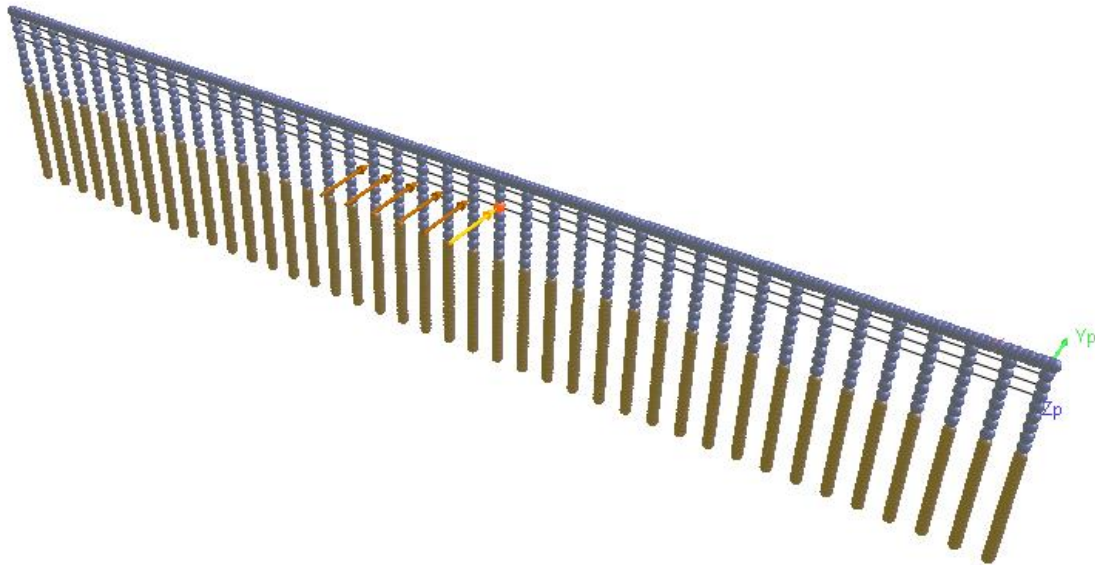
Figure 78: Layout – Load Case 10 (Section 3 – Soil C4)
