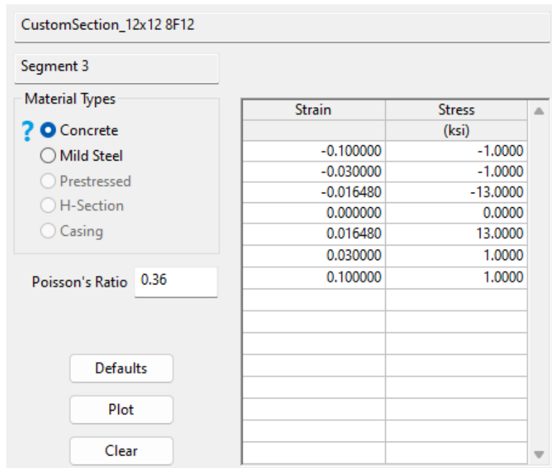
Figure 32: 12x12 8F12 Wale Properties
