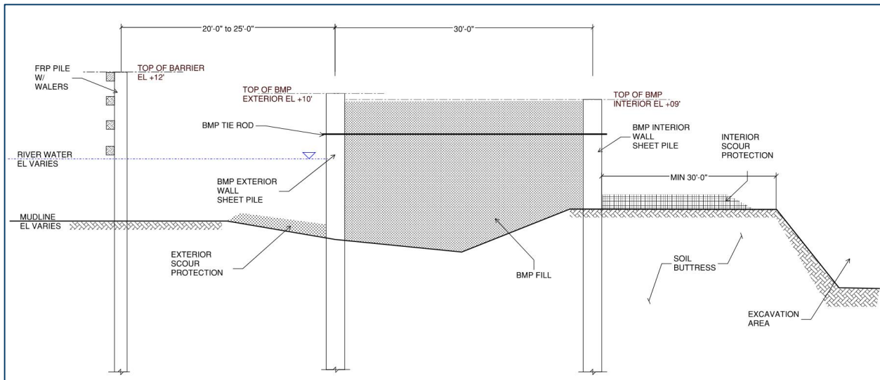
Figure 1.2 Typical Cross-Section of the BMP
