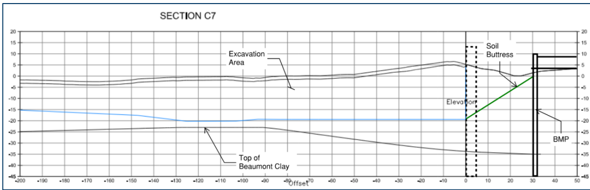
Figure 6.10 Analysis Section C7
