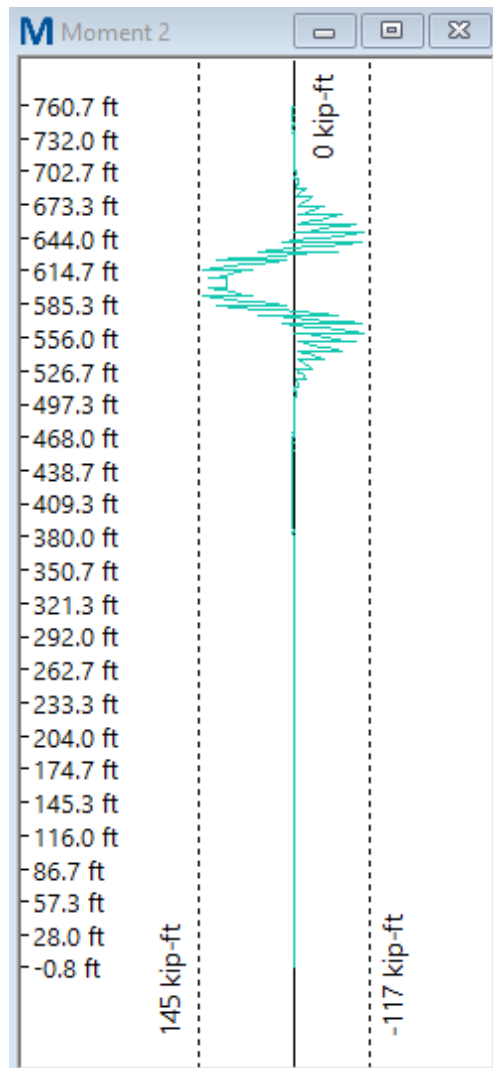
Figure 46: Max Wale Moment - Load Case 3 (Section 2 – Soil C4)
