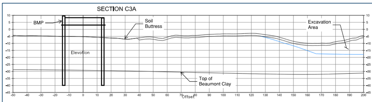
Figure 6.5 Analysis Section C3A
