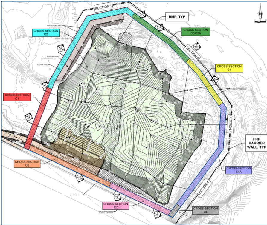
Figure 2.1 Alignment - FRP Barrier Wall
