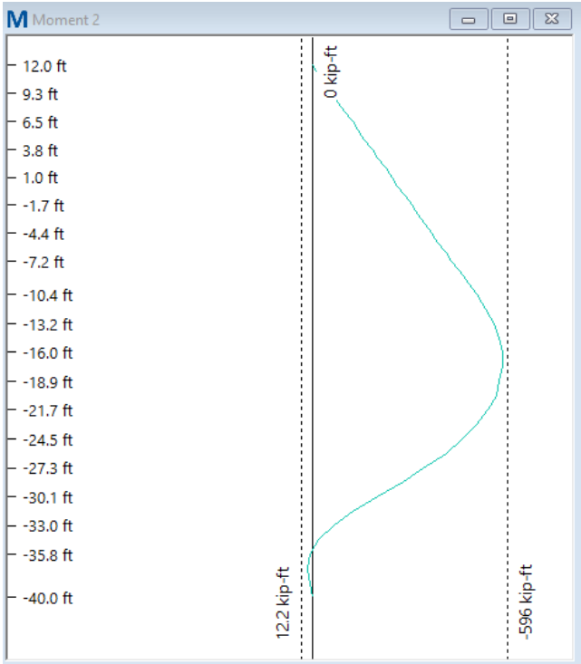
Figure 96: Moment Diagram Down the Elevation (Soil C3)
