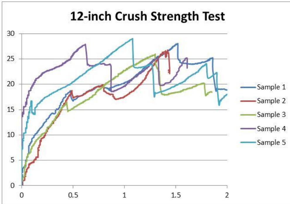
Figure 9: 12-inch Pile Crush Test Results
