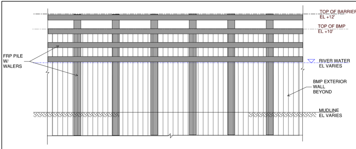
Figure 2.3 Typical Elevation - FRP Barrier Wall
