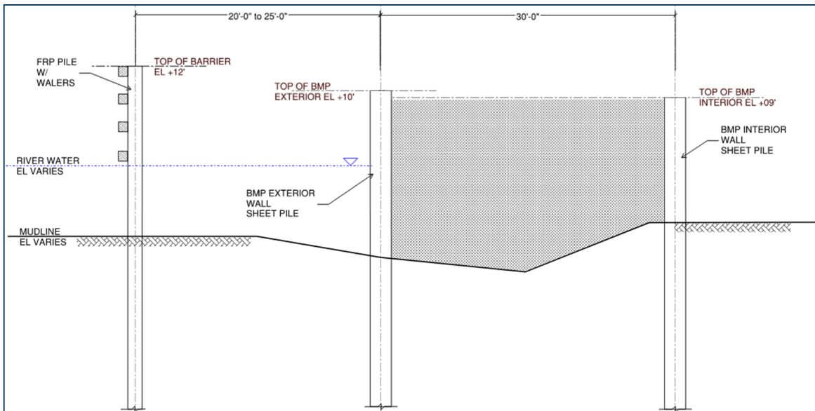
Figure 2.2 Typical Section - FRP Barrier Wall
