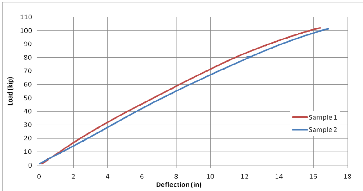
Figure 7: 16 inch Polyurethane Four-Point Bend Load-Deflection Response
