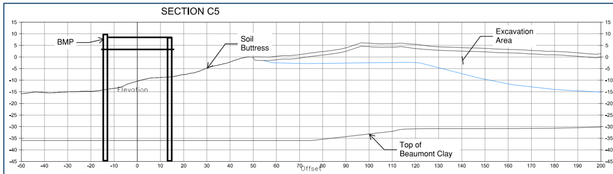
Figure 6.8 Analysis Section C5
