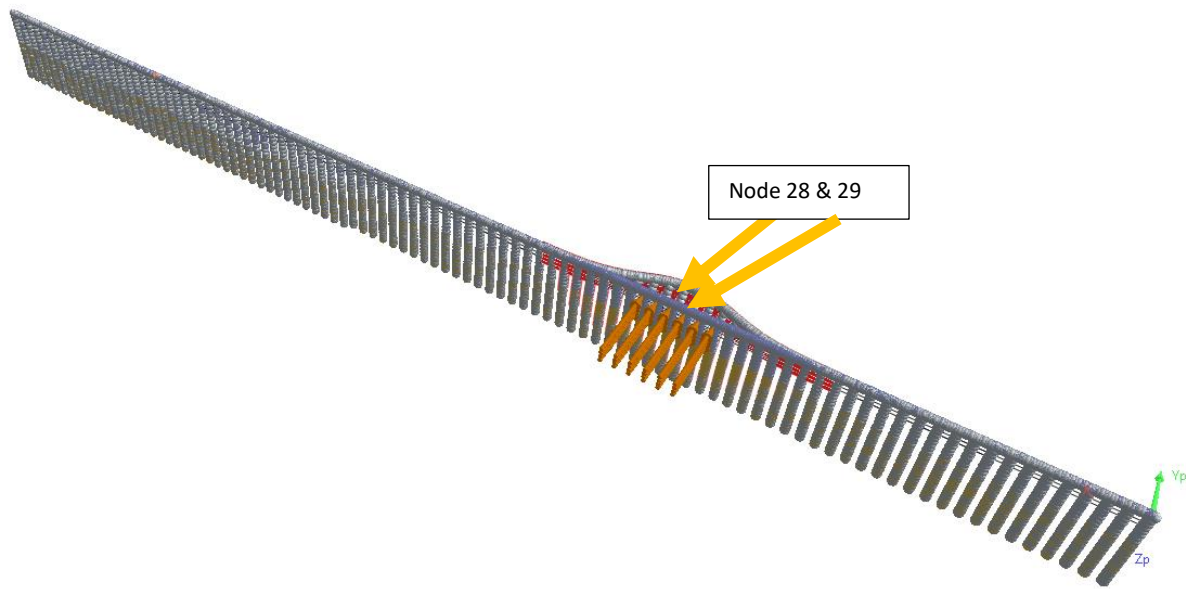
Figure 42: Displacement - Load Case 2 (Section 2 – Soil C3)
