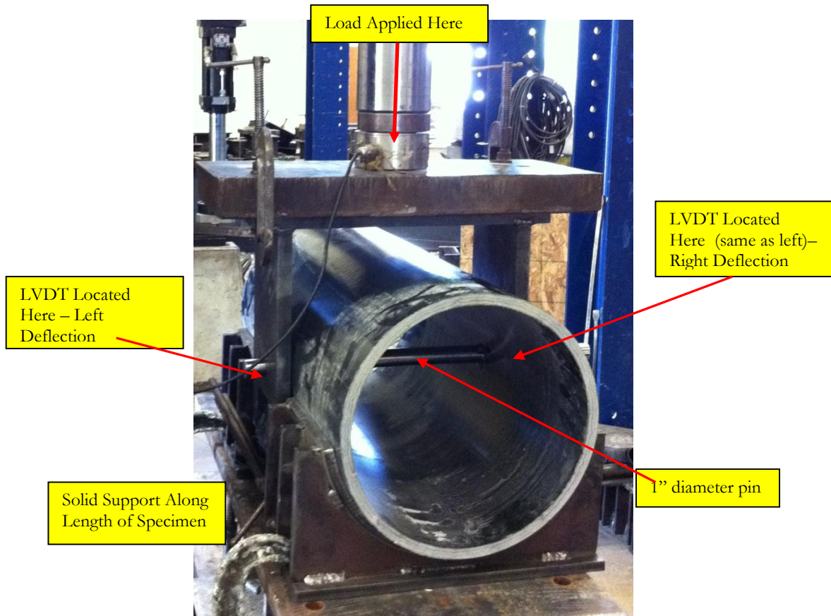
Figure 4: Connection Test A Setup
