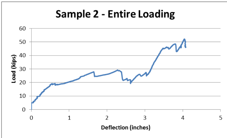
Figure 15: Sample 2 - Entire Loading
