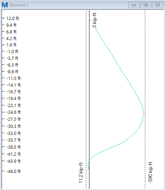
Figure 94: Moment Diagram Down the Elevation (Soil C2)
