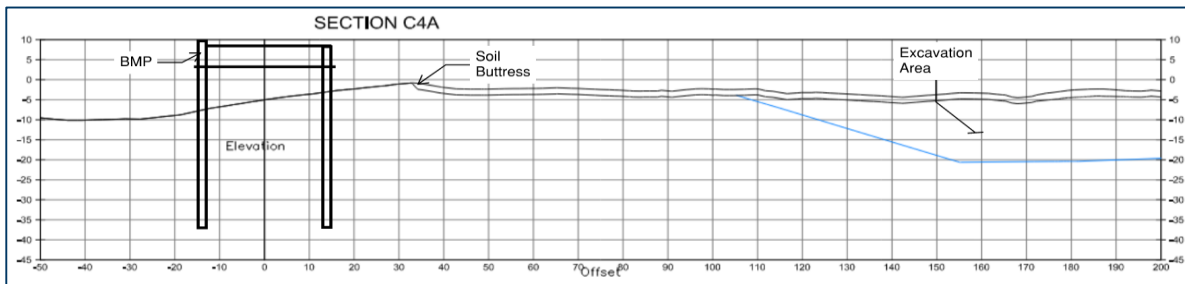
Figure 6.7 Analysis Section C4A
