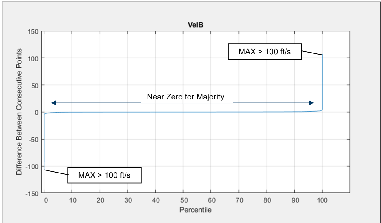
Figure 3 X-Direction Percentile Plot for Difference in Consecutive Points
