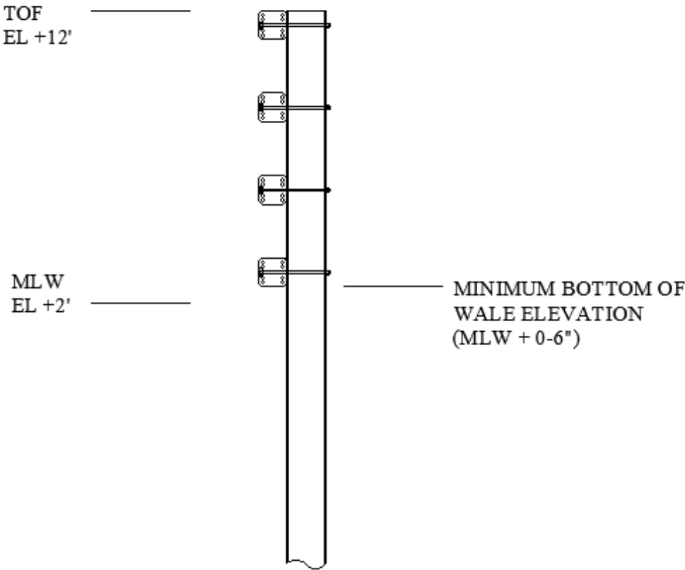
Figure 2: Fender Elevation
