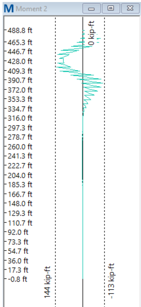
Figure 61: Max Wale Moment - Load Case 6 (Section 4 – Soil C5)
