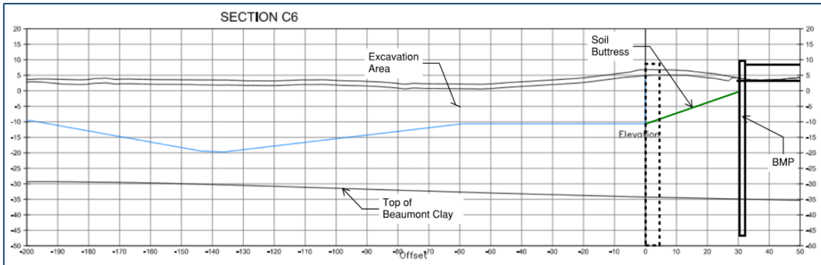
Figure 6.9 Analysis Section C6
