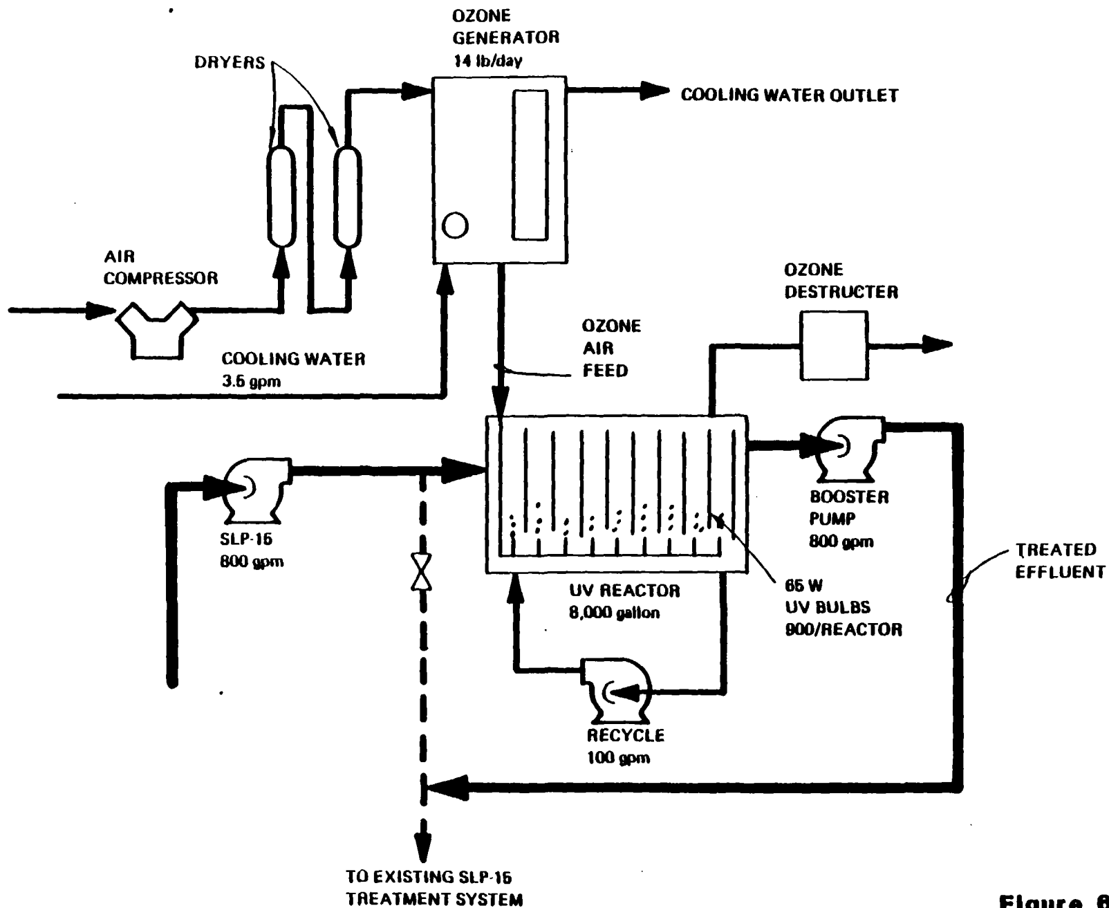
Figure 6-2 Ozone-UV Flow Diagram
