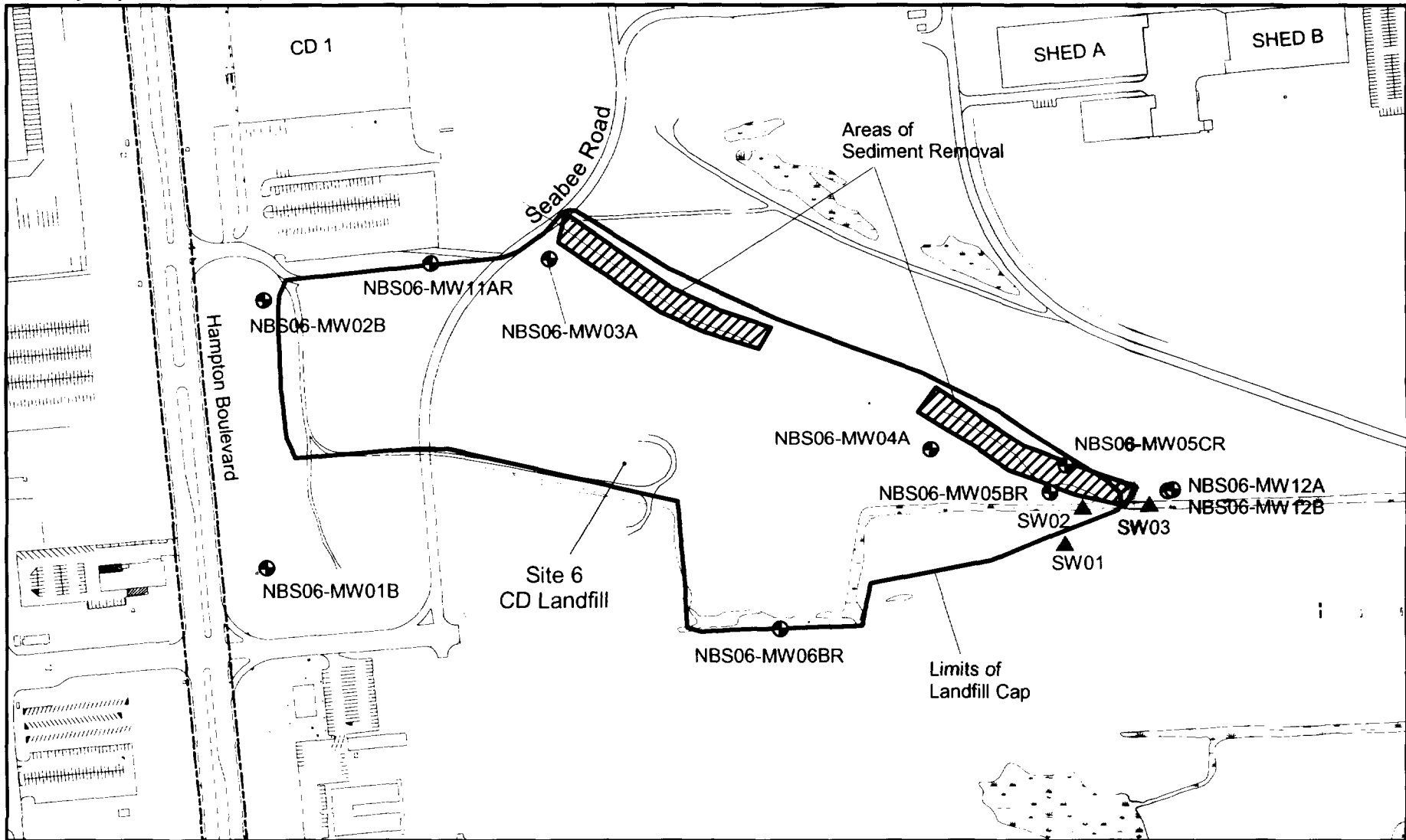
Figure 3-8 Areas of Sediment Removal and Landfill Cap Site 6 - CD Landfill Naval Station Norfolk Norfolk, Virginia
