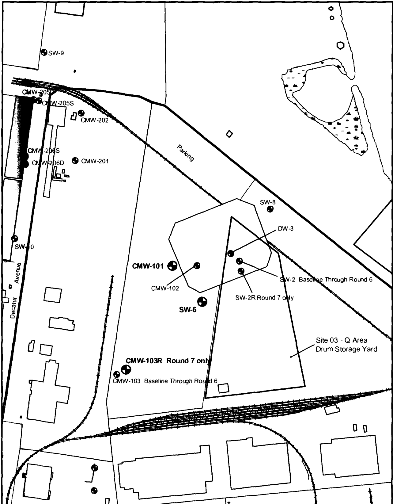
Figure 5-3 Monitoring Wells That Exceed Cleanup Criteria Q Area Drum Storage Yard - AOC 1 Long-Term Monitoring Program Naval Station Norfolk
