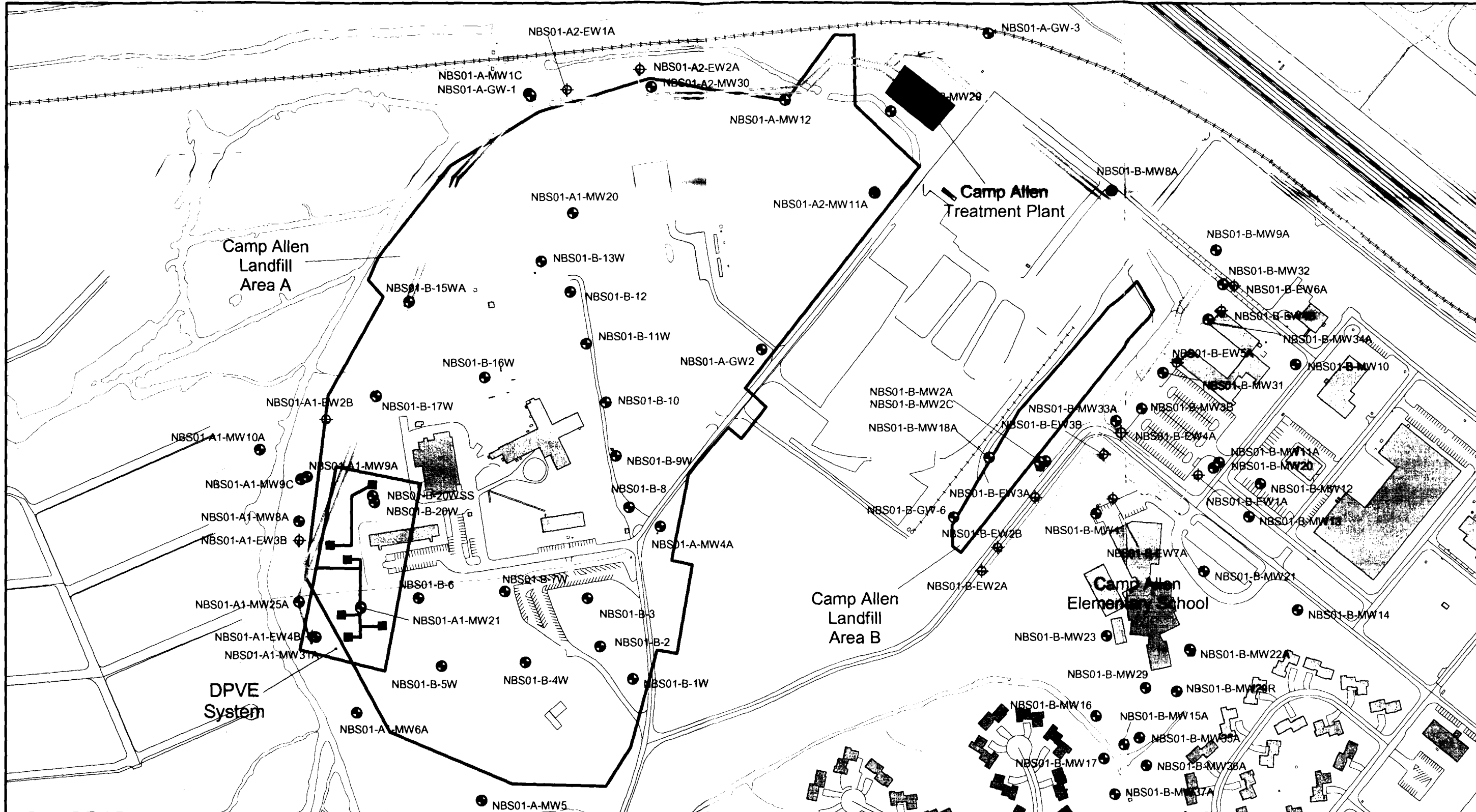
Figure 3-3 Layout of the Groundwater Extraction System and Shallow Monitoring Wells Site 1 - Camp Allen Landfill Naval Station Norfolk Norfolk, Virginia
