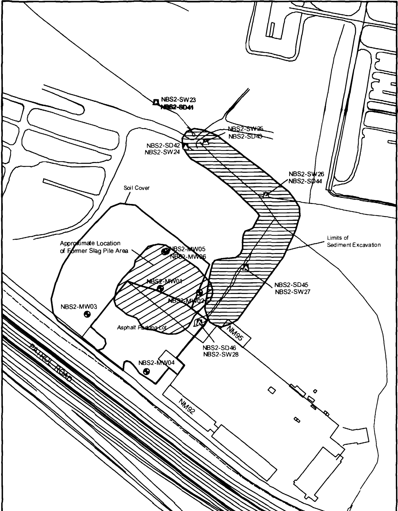
Figure 3-4 Soil Cover and Limits of Sediment Excavation Site 2 - Former NM Slag Pile Naval Station Norfolk Norfolk, Virginia
