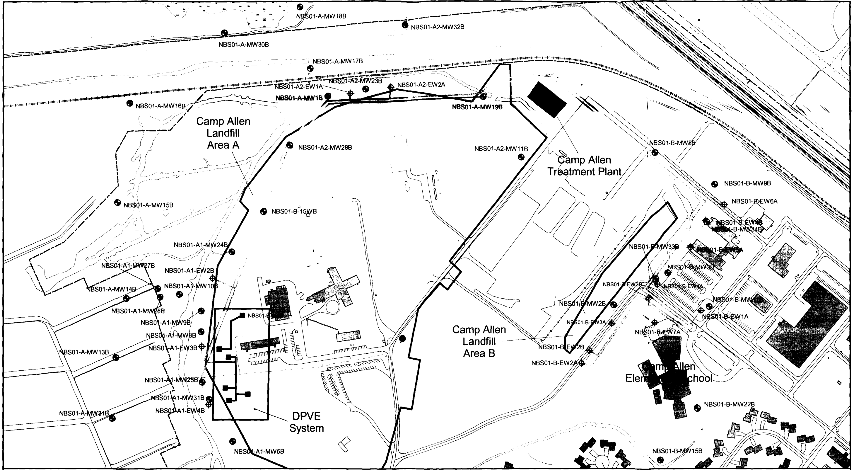
Figure 3-2 Layout of the Groundwater Extraction and Deep Monitoring Wells Site 1 - Camp Allen Landfill Naval Station Norfolk Norfolk, Virginia
