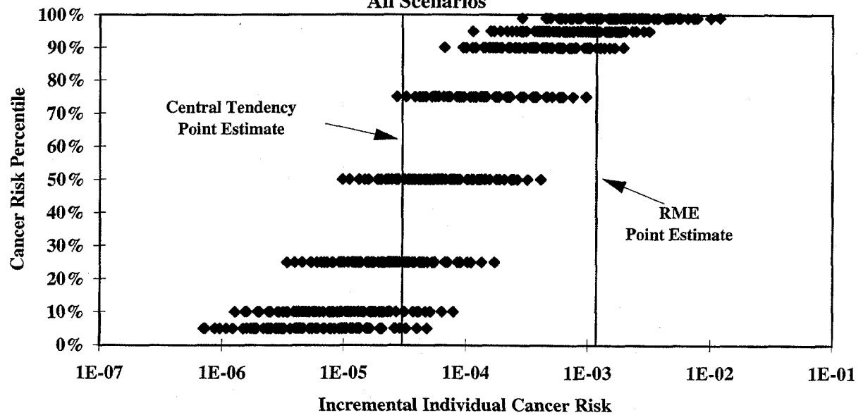
Figure 5-3b Monte Carlo Cancer Risk Summary All Scenarios
