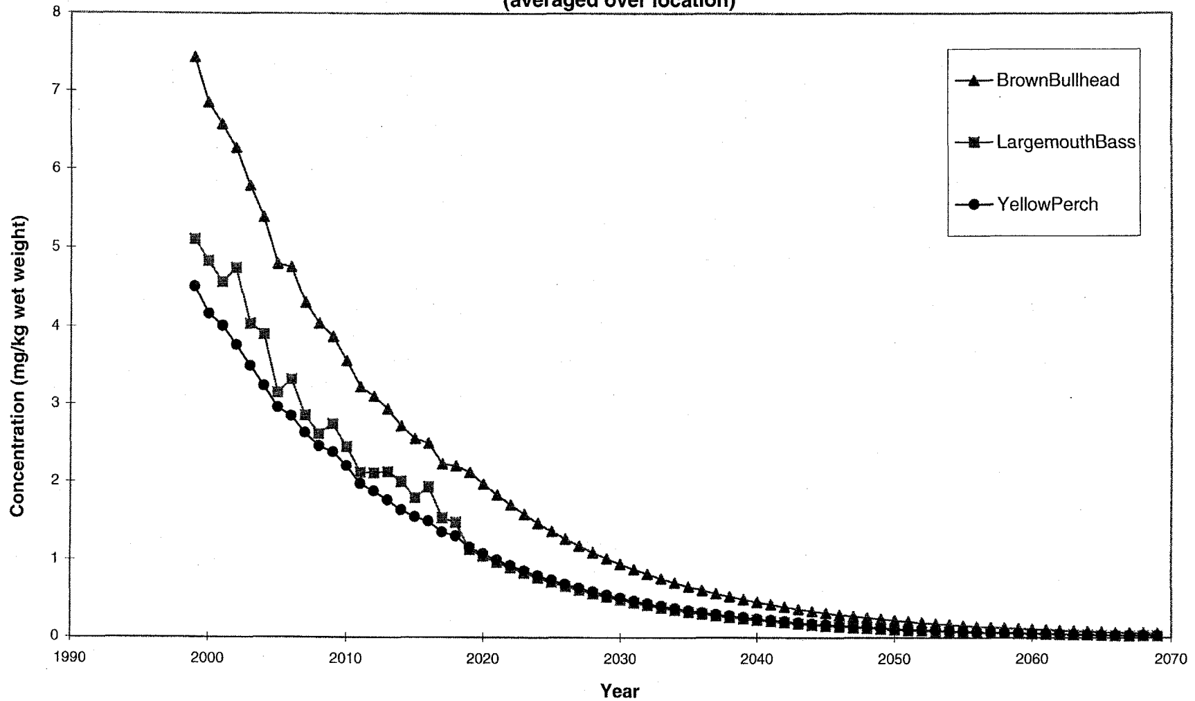
Figure 2-10 PCB Concentration by Species, 1999-2069 (averaged over location)
