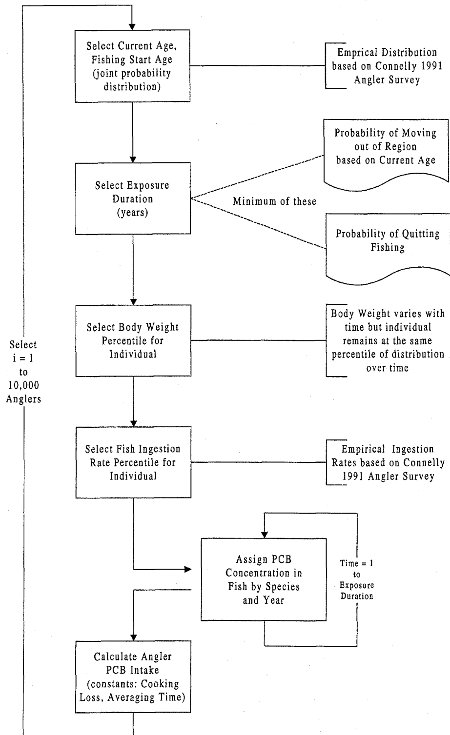
Figure 3-1 Diagram of Monte Carlo Simulation Process
