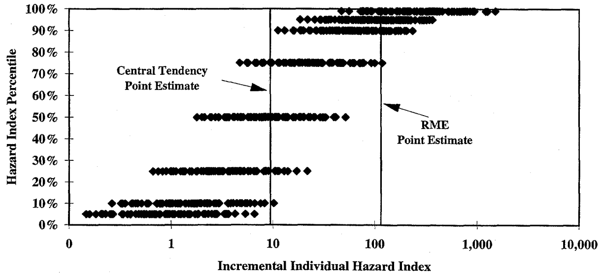
Figure 5-3a Monte Carlo Non-Cancer Hazard Index Summary All Scenarios
