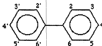
Figure 1: Basic Chemical Structure of PCBs
