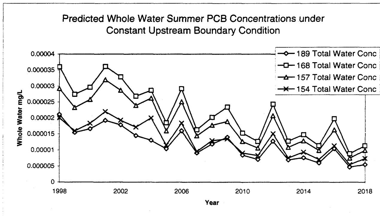
Figure 7.2 Predicted Concentrations from Fate and Transport Model under Constant Upstream Boundary Conditions
