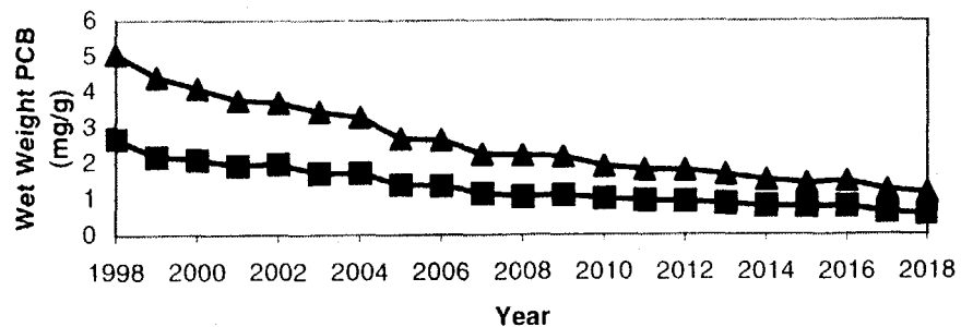
White Perch Predicted Wet Weight PCB Concentrations for River Mile 154: Prediction Period
