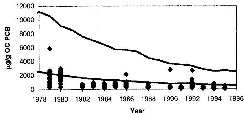
Brown Bullhead Lipid Normalized Concentrations for River Mile 189: Calibration Period
