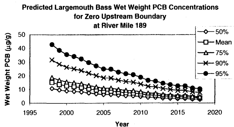
Figure 7-4 Predicted Wet Weight Concentrations Under Zero Upstream Boundary Condition from Empirical Probabilistic Model
