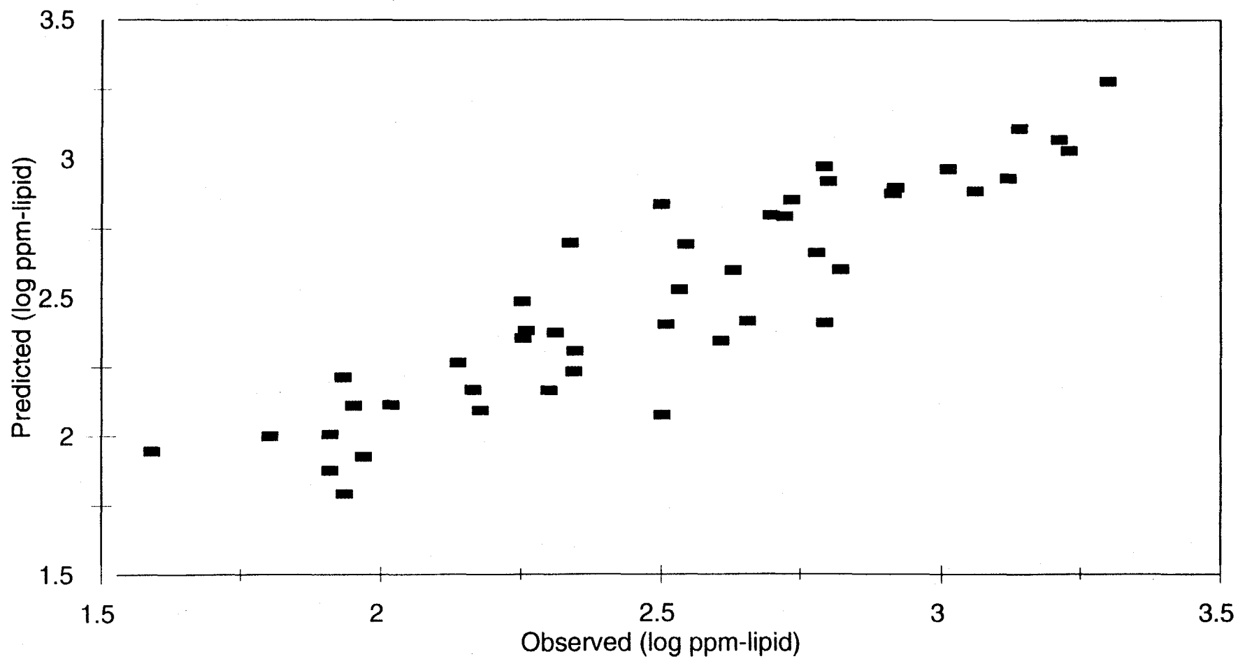
Figure 4-5 Observed versus Predicted Concentrations of \Sigma Tri+ PCBs for Brown Bullhead from Bivariate BAF Model
