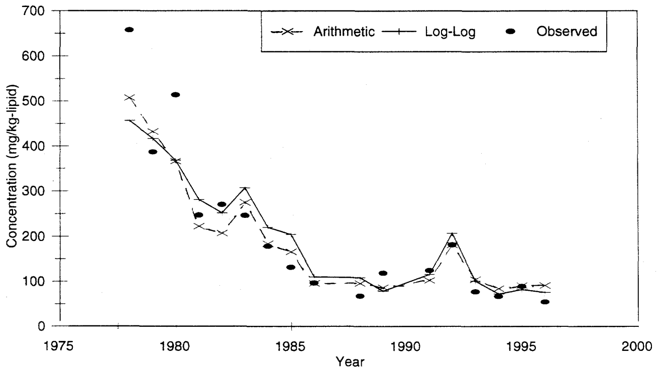
Figure 4-10 Comparison of Bivariate BAF Model Predictions and Observations of Mean Summer Body Burden of \Sigma Tri+ PCBs in Pumpkinseed
