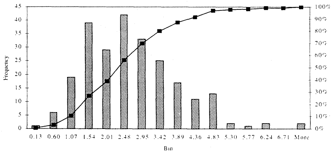
Cumulative Frequency of Largemouth Bass Ratios
