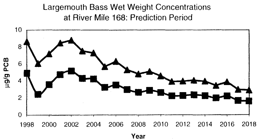
Figure 7-14 Predicted Wet Weight Concentrations From FISHRAND River Mile 168
