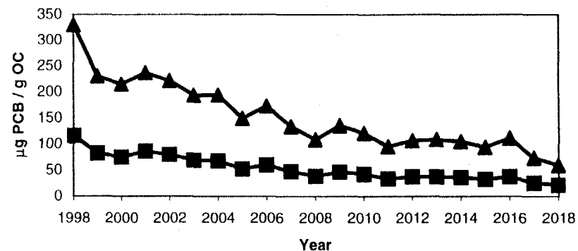
Yellow Perch Lipid Normalized Concentrations at River Mile 157: Prediction Period
