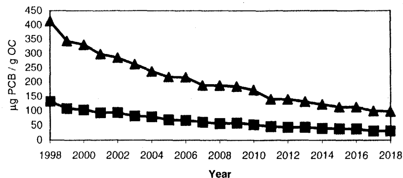
Yellow Perch Lipid Normalized Concentrations at River Mile 189: Prediction Period
