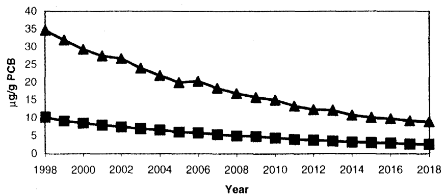
Brown Bullhead Wet Weight Concentrations for River Mile 189: Prediction Period
