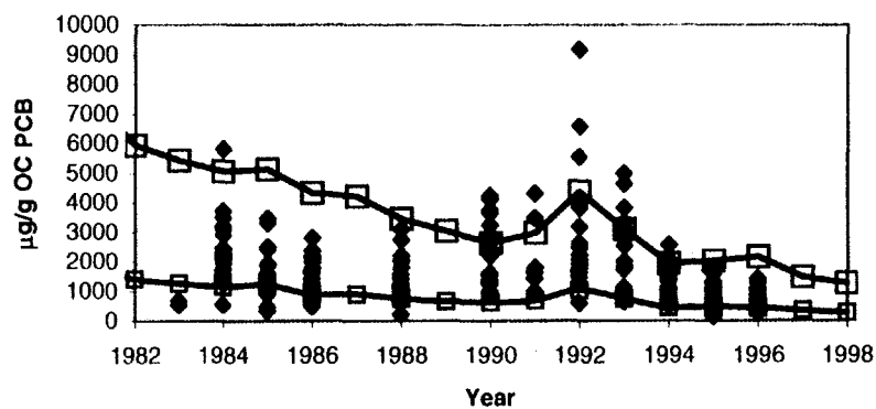
Largemouth Bass Lipid Normalized Concentrations at River Mile 189: Calibration Period
