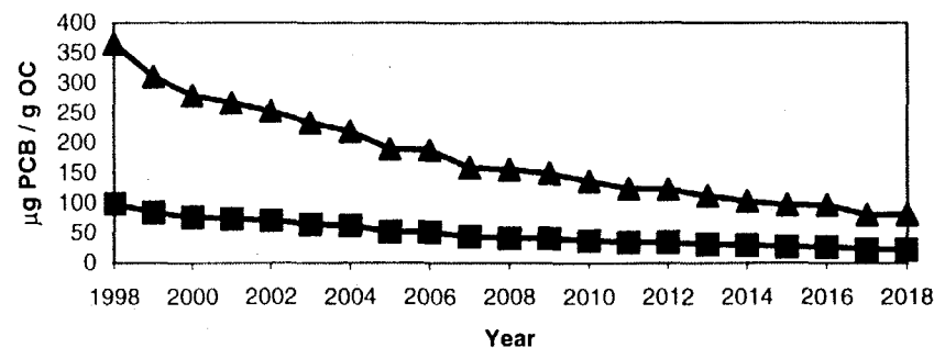
Brown Bullhead Lipid Normalized Concentrations for River Mile 154: Prediction Period
