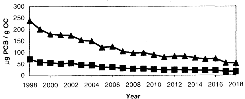
White Perch Lipid Normalized PCB Concentrations for River Mile 157: Prediction Period
