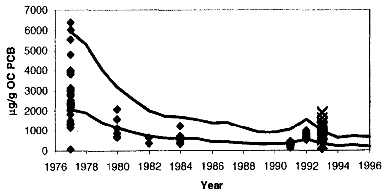
Yellow Perch Lipid Normalized Concentrations at River Mile 189: Calibration Period
