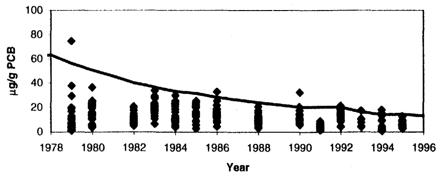
Brown Bullhead Wet Weight Concentrations for River Mile 189: Calibration Period
