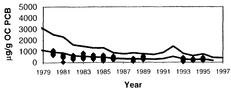
Pumpkinseed Lipid Normalized Concentrations for River Mile 168
