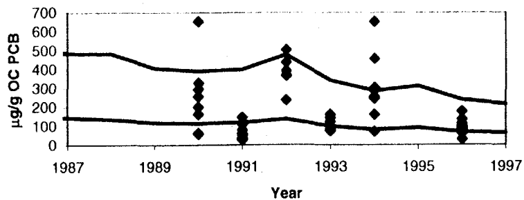
White Perch Lipid Normalized Concentrations for River Mile 152-154: Calibration Period
