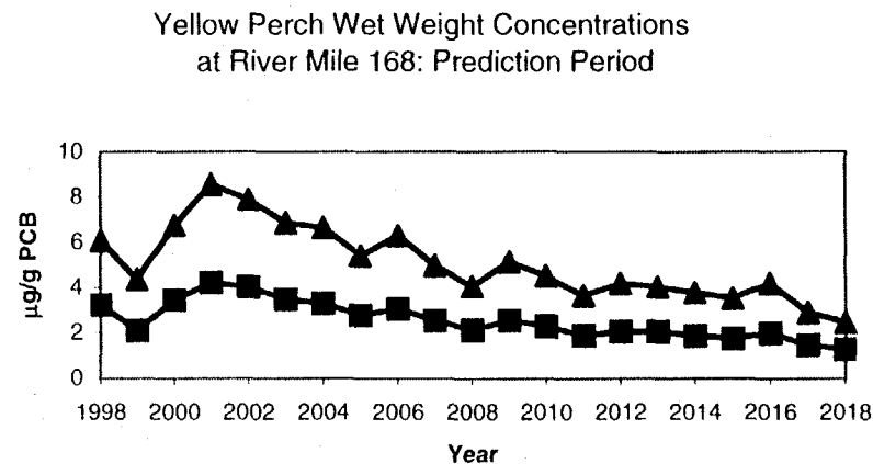
Figure 7-14 Predicted Wet Weight Concentrations From FISHRAND River Mile 168
