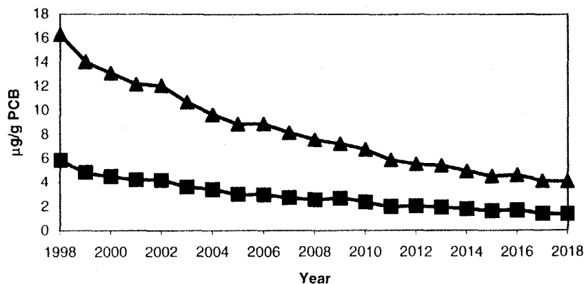
Largemouth Bass Wet Weight Concentrations at River Mile 189: Prediction Period
