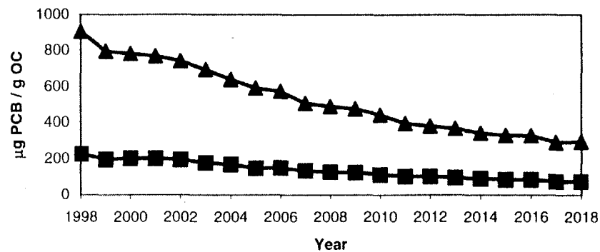
Brown Bullhead Lipid Normalized Concentrations for River Mile 168: Prediction Period
