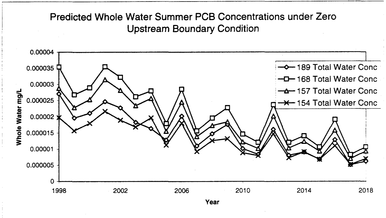
Figure 7.1 Predicted Concentrations from Fate and Transport Model under Zero Upstream Boundary Conditions
