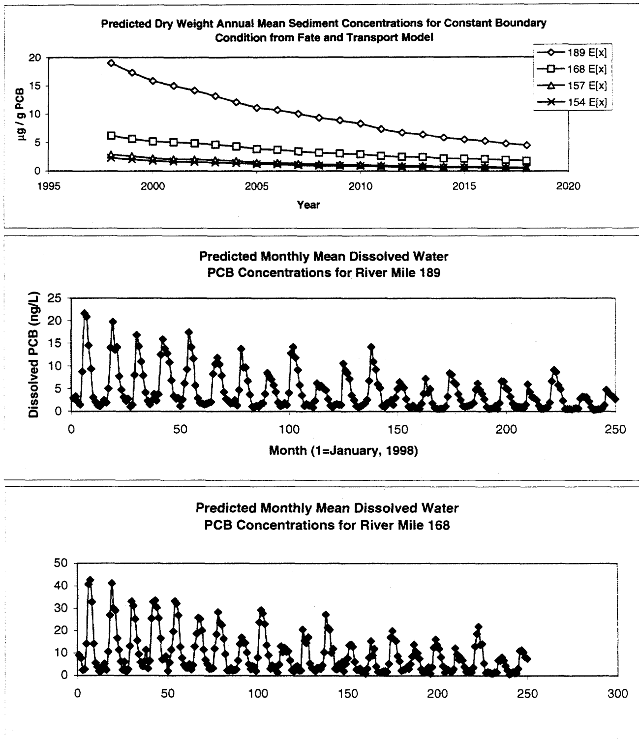
Figure 7-9 Predicted Dissolved Water and Dry Weight Sediment Concentrations under Zero Boundary Condition
