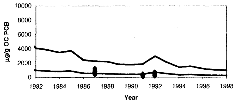
White Perch Lipid Normalized Concentrations for River Mile 157: Calibration Period
