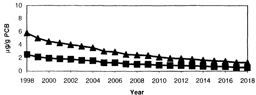
Brown Bullhead Wet Weight Concentrations for River Mile 154: Prediction Period
