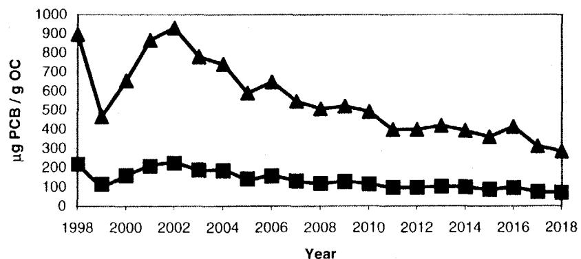
Largemouth Bass Lipid Normalized Concentrations at River Mile 168: Prediction Period
