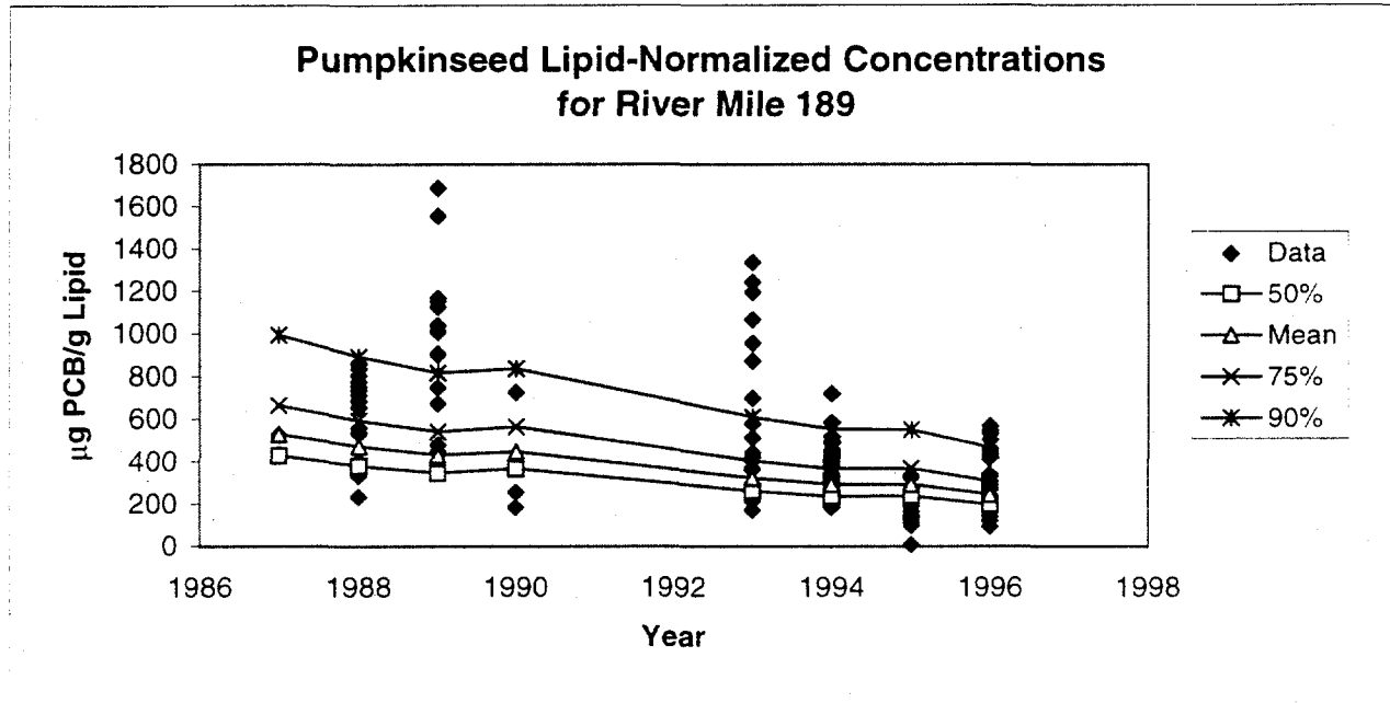
Figure 5-8 Probabilistic Empirical Model Calibration Results Using Output from Fate and Transport Model (for Pumpkinseed)
