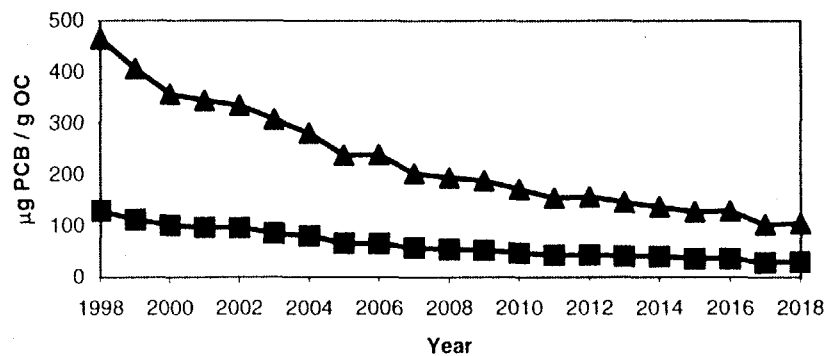
Brown Bullhead Lipid Normalized Concentrations for River Mile 157: Prediction Period
