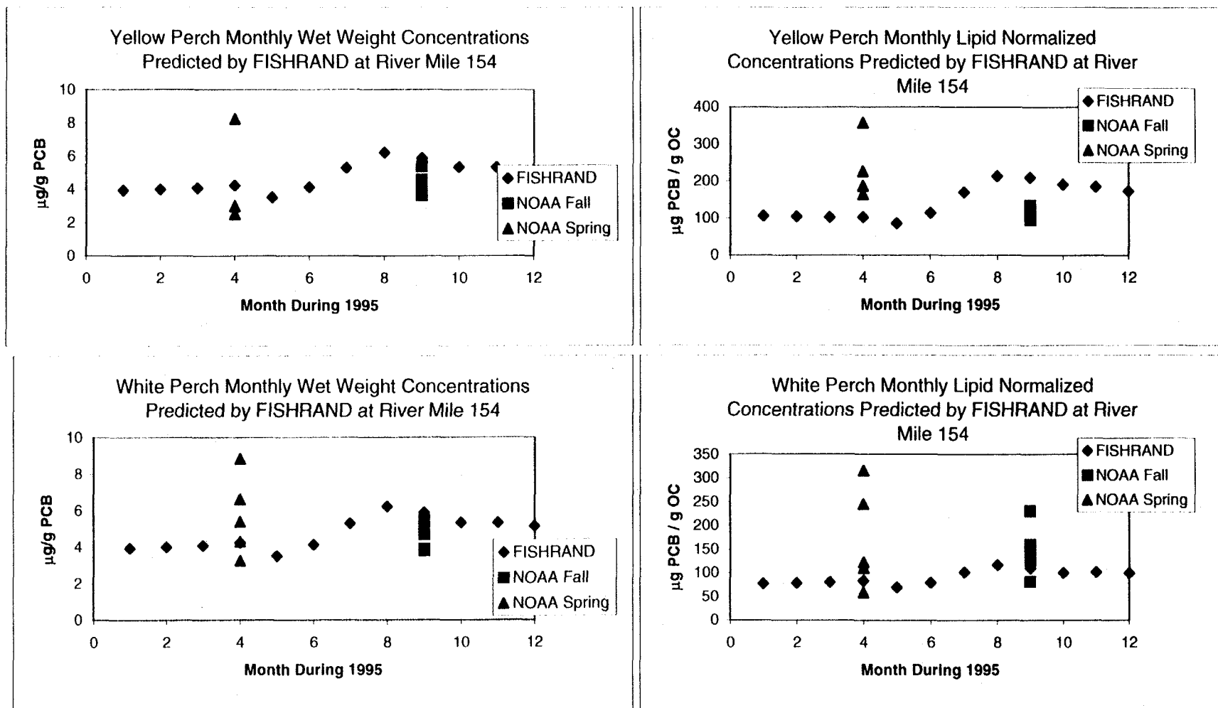
Figure 6-5 Seasonal Differences in Yellow And White Perch
