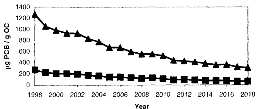
Largemouth Bass Lipid Normalized Concentrations at River Mile 189: Prediction Period
