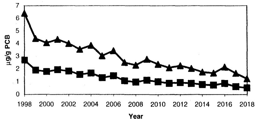
Yellow Perch Wet Weight Concentrations at River Mile 154: Prediction Period
