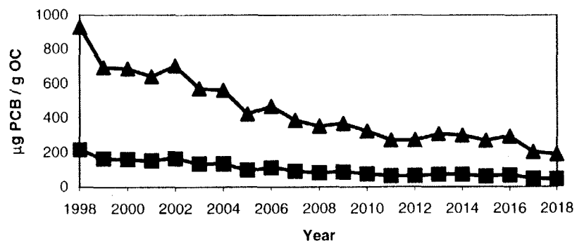
Largemouth Bass Lipid Normalized Concentrations at River Mile 157: Prediction Period
