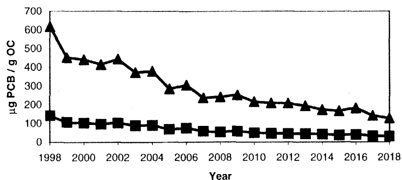
Largemouth Bass Lipid Normalized Concentrations at River Mile 154: Prediction Period
