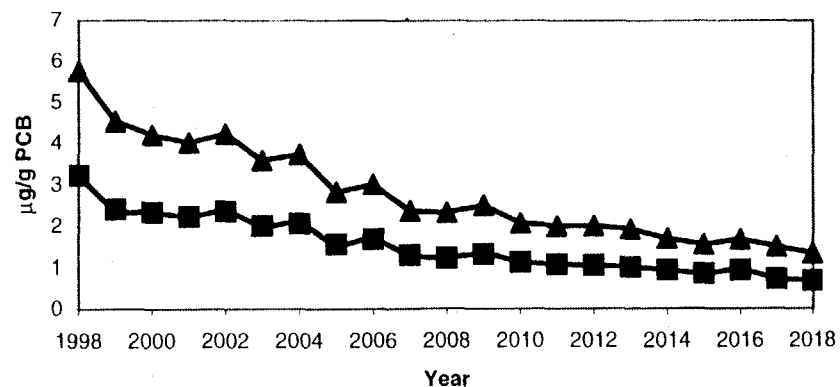
Largemouth Bass Wet Weight Concentrations at River Mile 154: Prediction Period
