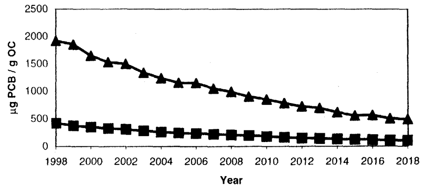
Brown Bullhead Lipid Normalized Concentrations for River Mile 189: Prediction Period
