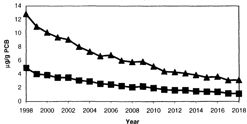
Yellow Perch Wet Weight Concentrations at River Mile 189: Prediction Period
