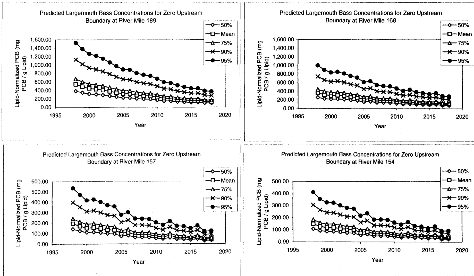
Figure 7-3 Predicted Lipid Normalized Concentrations under Zero Upstream Boundary Conditions from Empirical Probabilistic Model
