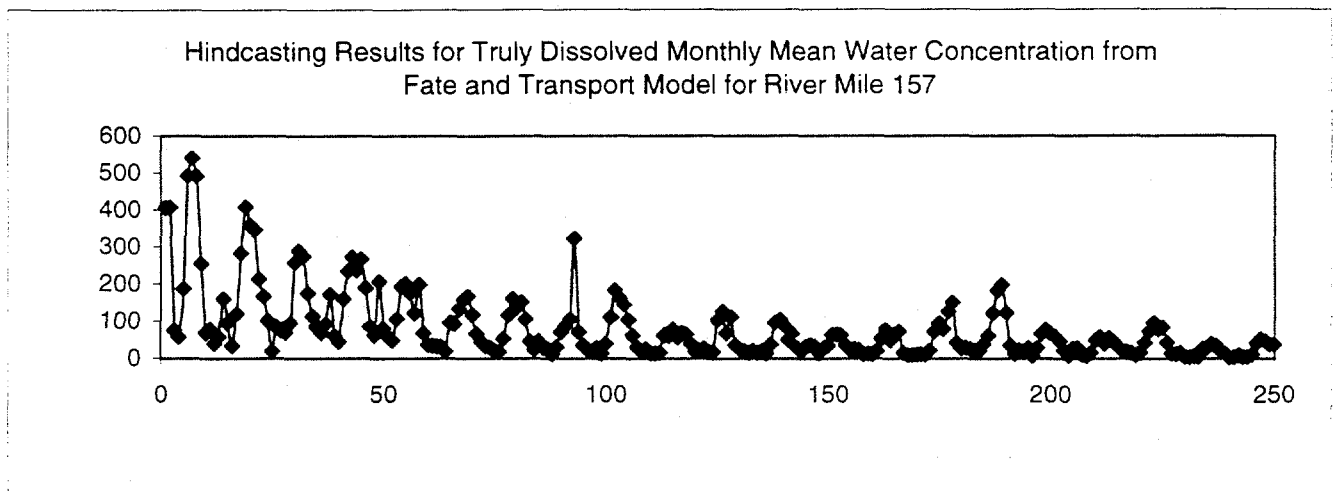
Figure 6-1 Hindcasting Concentrations From Fate And Transport Modeling For Water And Sediment (cont.)
