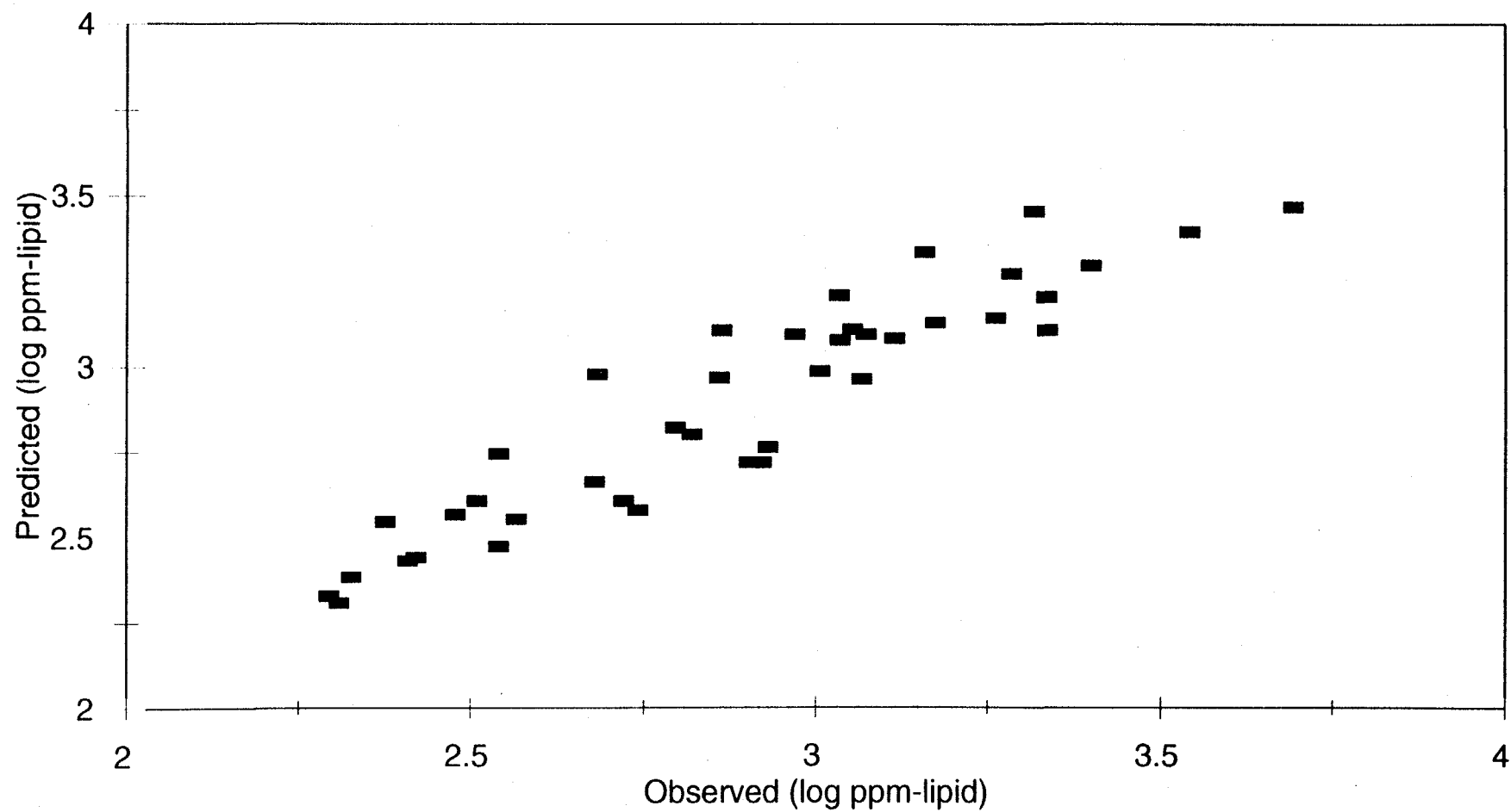
Figure 4-6 Observed versus Predicted Concentrations of \Sigma Tri+ PCBs for Largemouth Bass from Bivariate BAF Model
