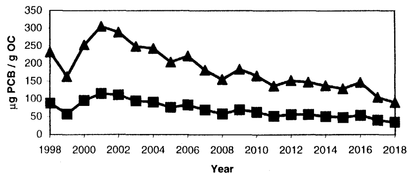
Yellow Perch Lipid Normalized Concentrations at River Mile 168: Prediction Period
