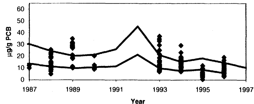
Pumpkinseed Wet Weight Concentrations for River Mile 189: Calibration Period
