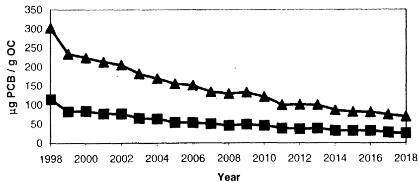
Pumpkinseed Lipid Normalized Concentrations for River Mile 189: Prediction Period
