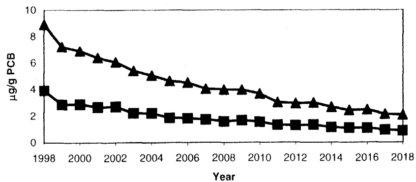
Pumpkinseed Wet Weight Concentrations for River Mile 189: Prediction Period
