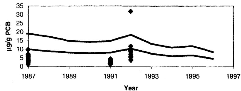
White Perch Wet Weight Concentrations for River Mile 157: Calibration Period
