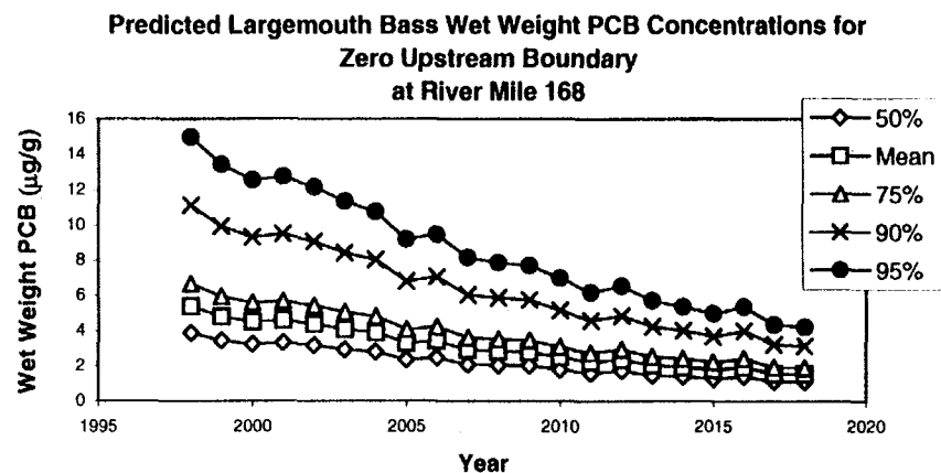
Figure 7-4 Predicted Wet Weight Concentrations Under Zero Upstream Boundary Condition from Empirical Probabilistic Model
