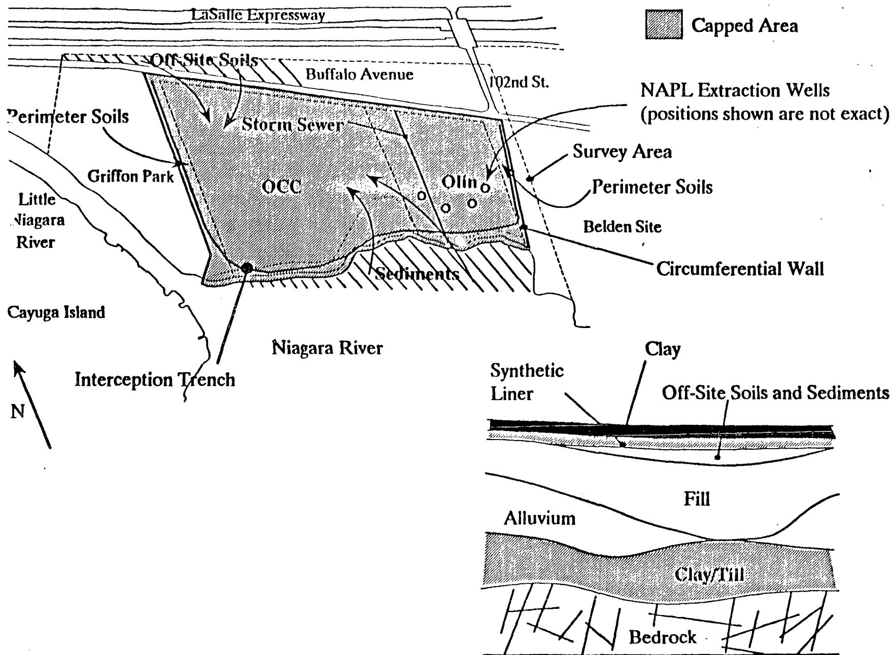
Figure 4 102nd Street Landfill Remedy -- Schematic
