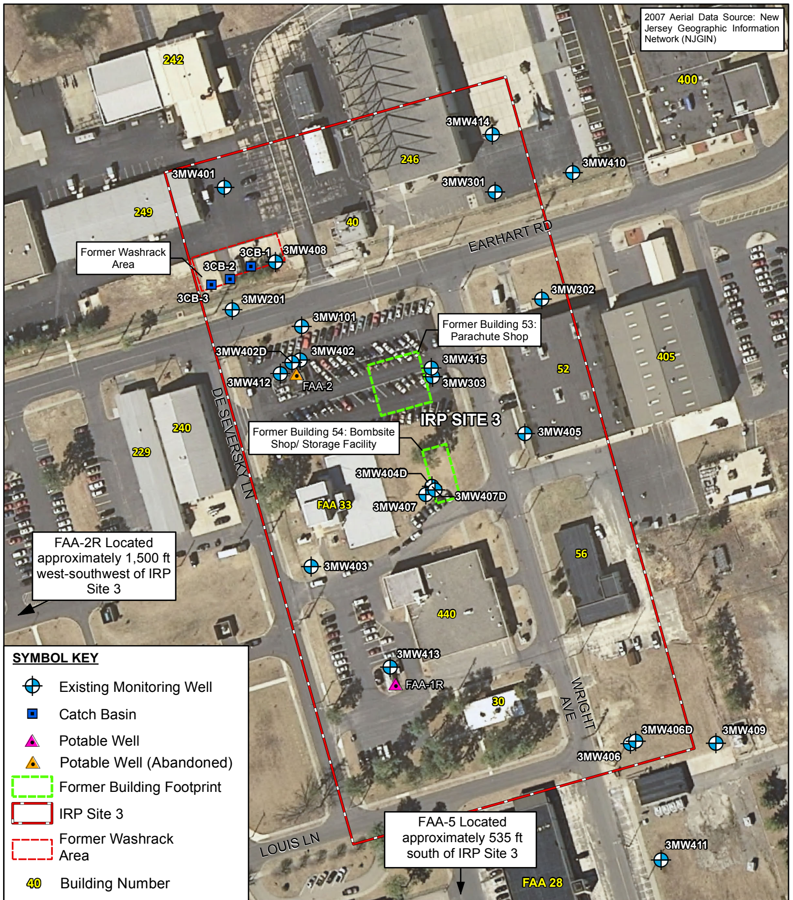
Figure 9 NJANG Site 3 Layout and Monitoring Well Locations
