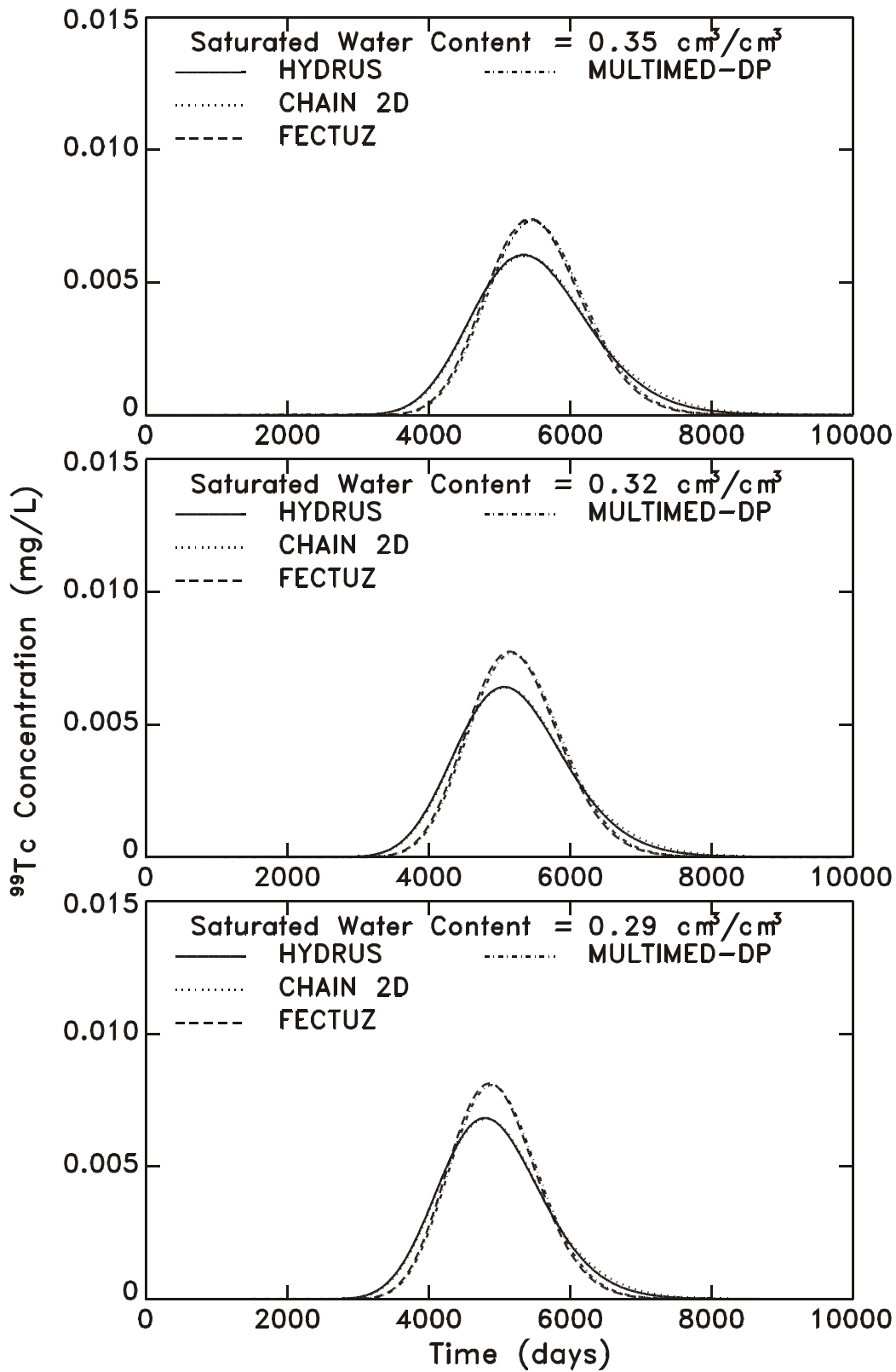
Figure 7-9. Sensitivity of ^{99}\text{Tc} breakthrough (through the 6m layer) to the saturated water content using the MULTIMED-DP 1.0, FECTUZ, CHAIN 2D and HYDRUS Models, where \theta_s = 0.35 \text{ cm}^3/\text{cm}^3 , 0.32 \text{ cm}^3/\text{cm}^3 , and 0.29 \text{ cm}^3/\text{cm}^3 .
