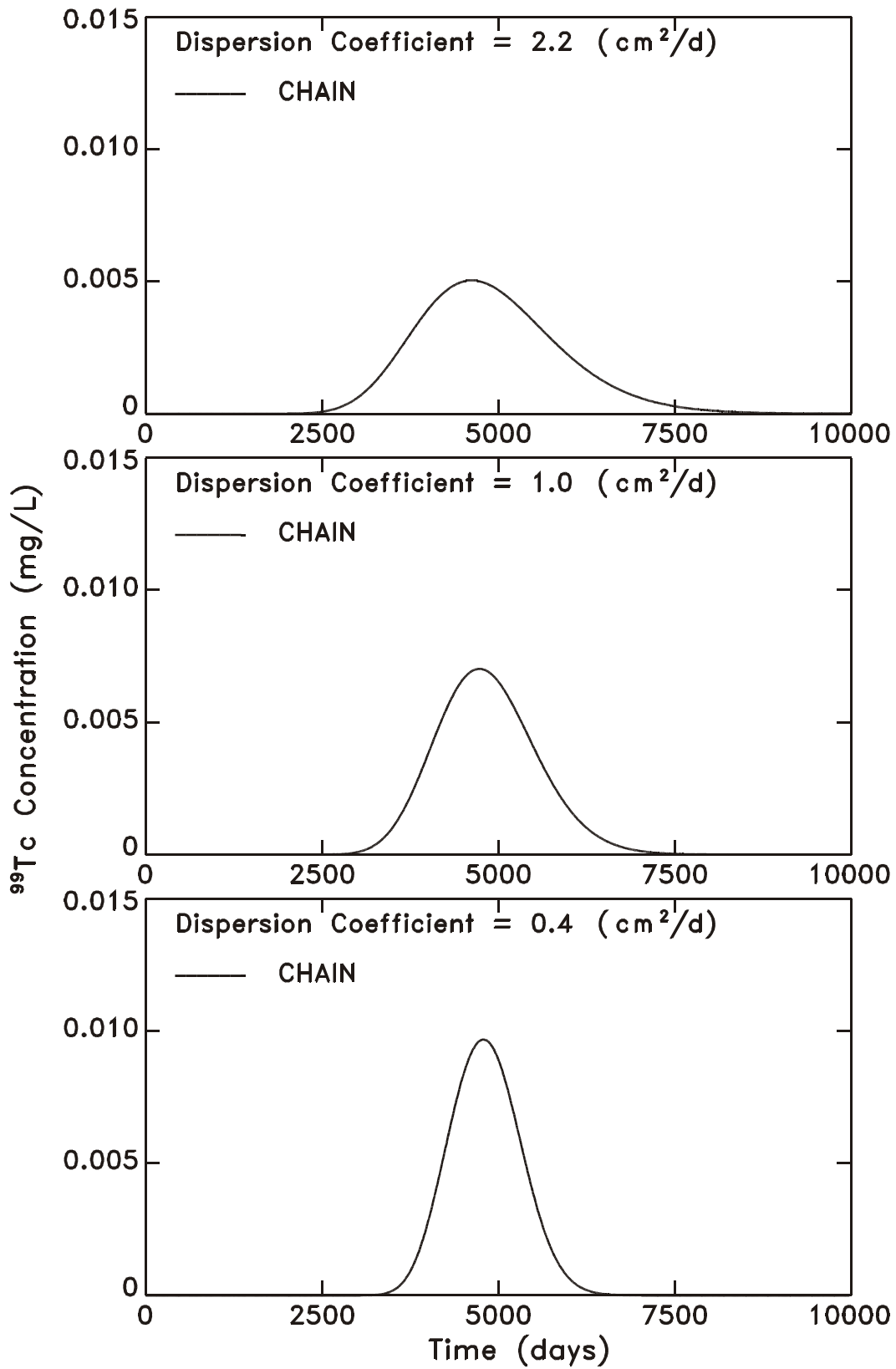
Figure 7-5. Sensitivity of 99 Tc breakthrough (through the 6m layer) to the dispersion coefficient using the CHAIN Model, where D = 2.20 \text{ cm}^2/\text{d} , 1.00 \text{ cm}^2/\text{d} , and 0.40 \text{ cm}^2/\text{d} .
