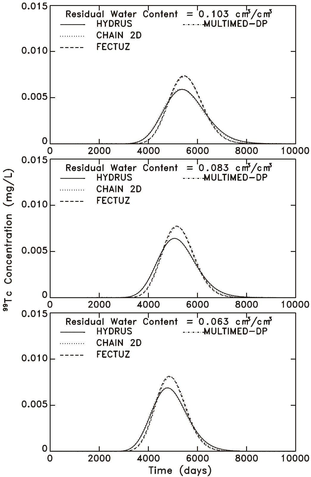
Figure 7-10. Sensitivity of ^{99}\text{Tc} breakthrough (through the 6m layer) to the residual water content using the MULTIMED-DP 1.0, FECTUZ, CHAIN 2D and HYDRUS Models, where \theta_r = 0.103 \text{ cm}^3/\text{cm}^3 , 0.083 \text{ cm}^3/\text{cm}^3 , and 0.063 \text{ cm}^3/\text{cm}^3 .
