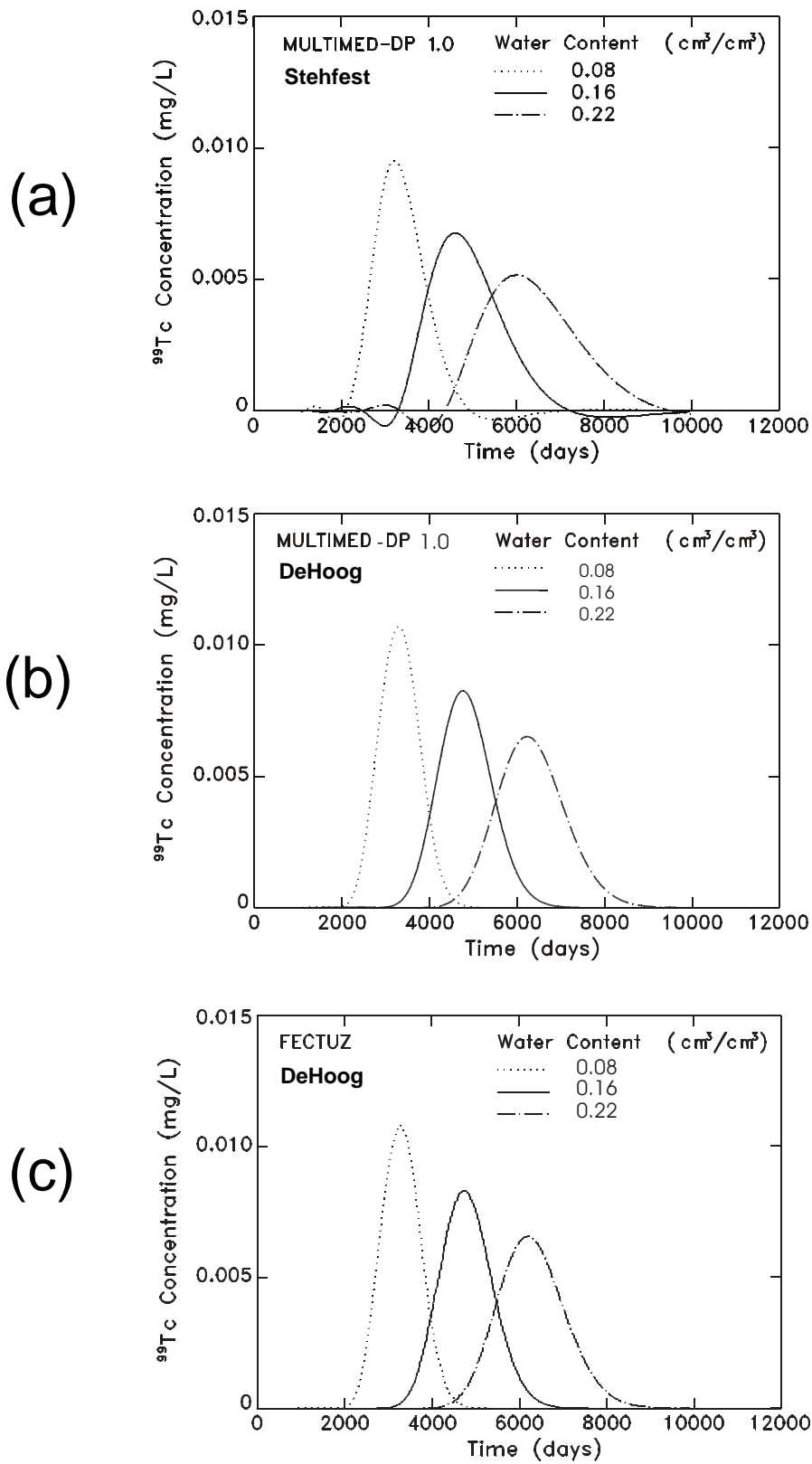
Figure 7-26. Sensitivity of 99 Tc BTCs at 6m depth to water content, where (a) uses Stehfest Algorithm of MULTIMED-DP 1.0, (b) uses DeHoog Algorithm of MULTIMED-DP 1.0, and (c) uses DeHoog Algorithm of FECTUZ Code.
