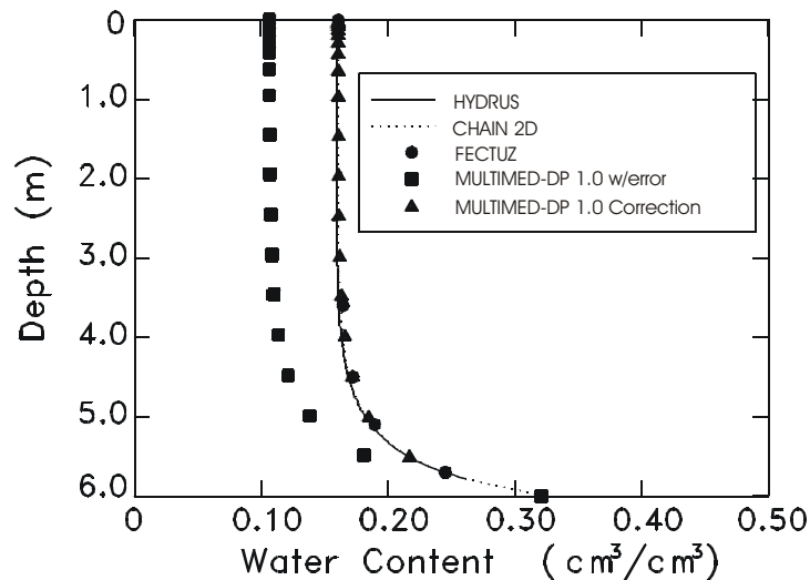
Figure 7-25. Water content distributions predicted by the HYDRUS, CHAIN 2D, FECTUZ, and MULTIMED-DP 1.0 models. Note that the water contents (■) obtained from the originally distributed MULTIMED-DP 1.0 code are in error. The corrected code gives a consistent water content distribution (▲) with the other three models.
