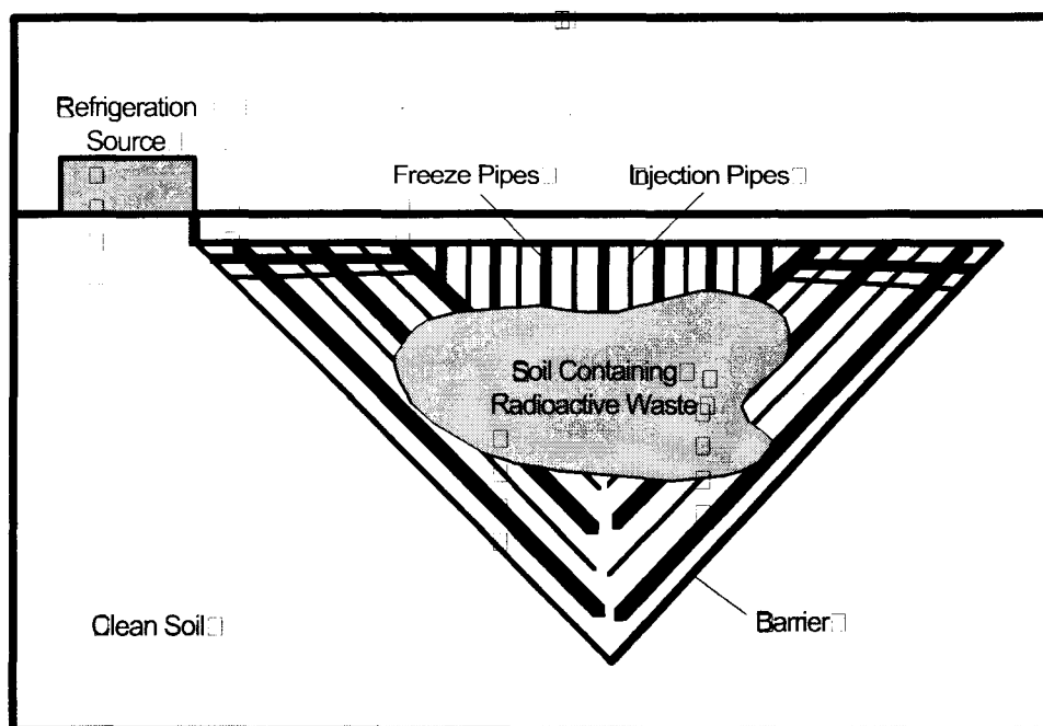
Exhibit 2-6: Cryogenic Barrier
