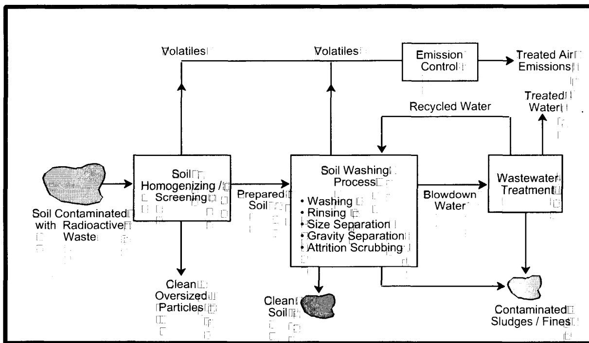
Exhibit 2-20: Soil Washing
