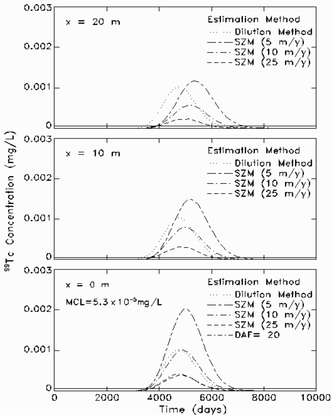
Figure 3.4. Base case predication of ^{99}\text{Tc} concentration at the receptor well by employing dilution factor method and using saturated zone model (SZM) -- FECTUZ. The numbers in the parentheses are ground water velocity. The solid lines are used to represent the MCL ( 5.3 \times 10^{-5} mg/L) level.
