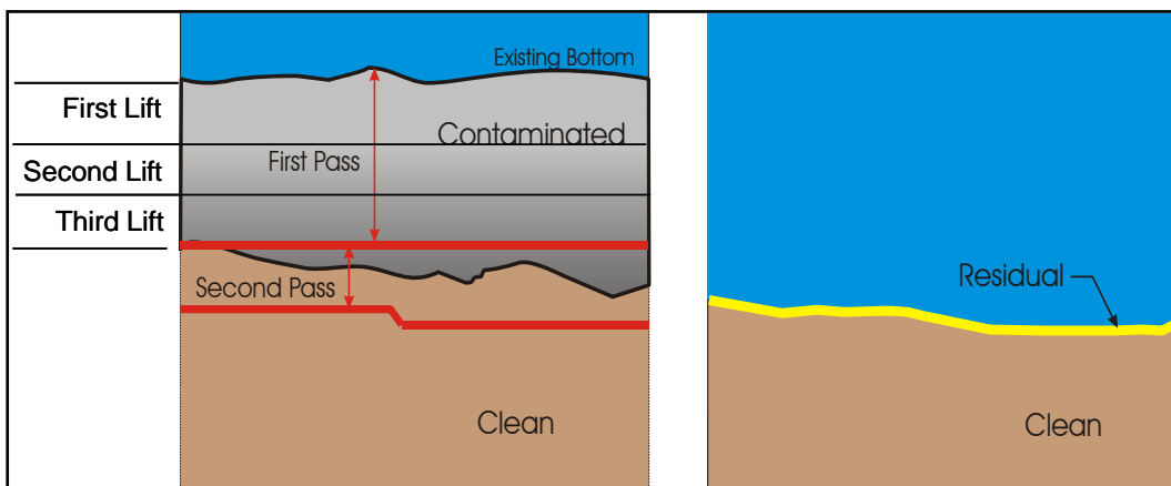
Figure 23. Multiple dredge passes, each lift not to exceed 3 to 5 ft. (Source: Dalton, Olmsted & Fuglevand).
