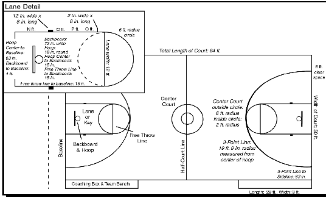
Exhibit A-11 Basketball Court Diagram (adapted from Pioneer Manufacturing Co.)
