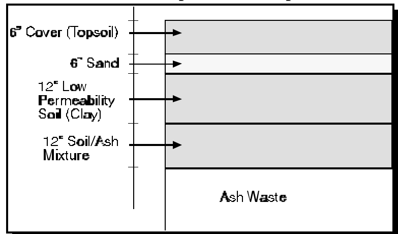
Cross-Section Diagram of the Chisman Creek Superfund Site Cap
