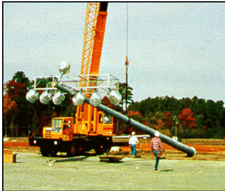
Workers install lights for sports fields during construction of the cover system at the Chisman Creek Superfund site in Yorktown, Virginia, a former fly ash disposal area.
