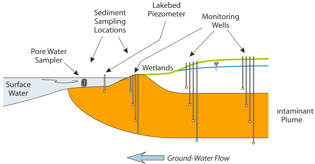
Figure 10. Conceptual monitoring network for verifying lack of impact to ground-water discharge.
