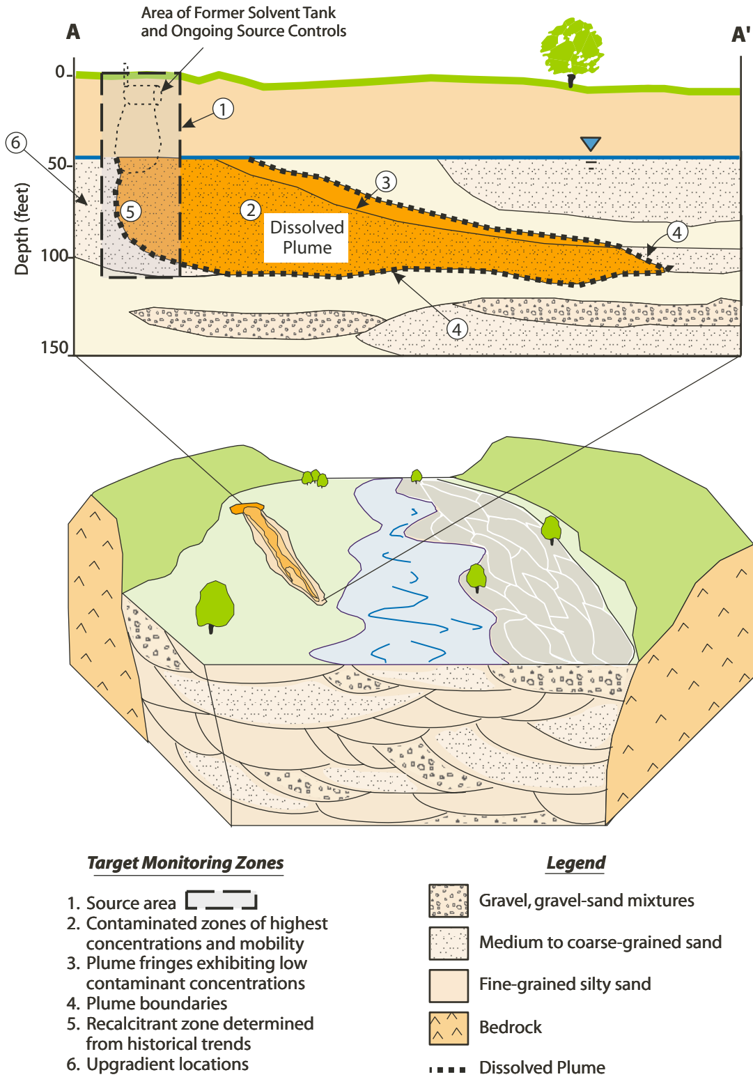
Figure 3. Geologic block diagram and cross section depicting a stream environment in which sediments have accumulated as valley fill. In the figure, there are numerous coarse-grained deposits as well as finer-grained materials with lower hydraulic conductivity.
