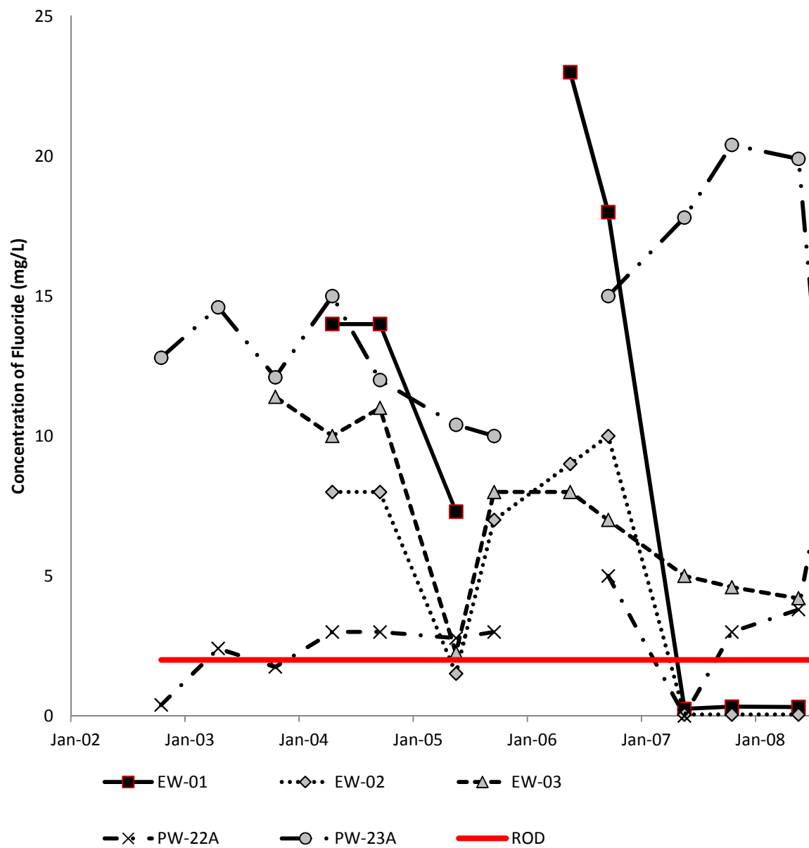
Figure 6-3. Concentration of Fluoride (F) in Groundwater in the FMA
