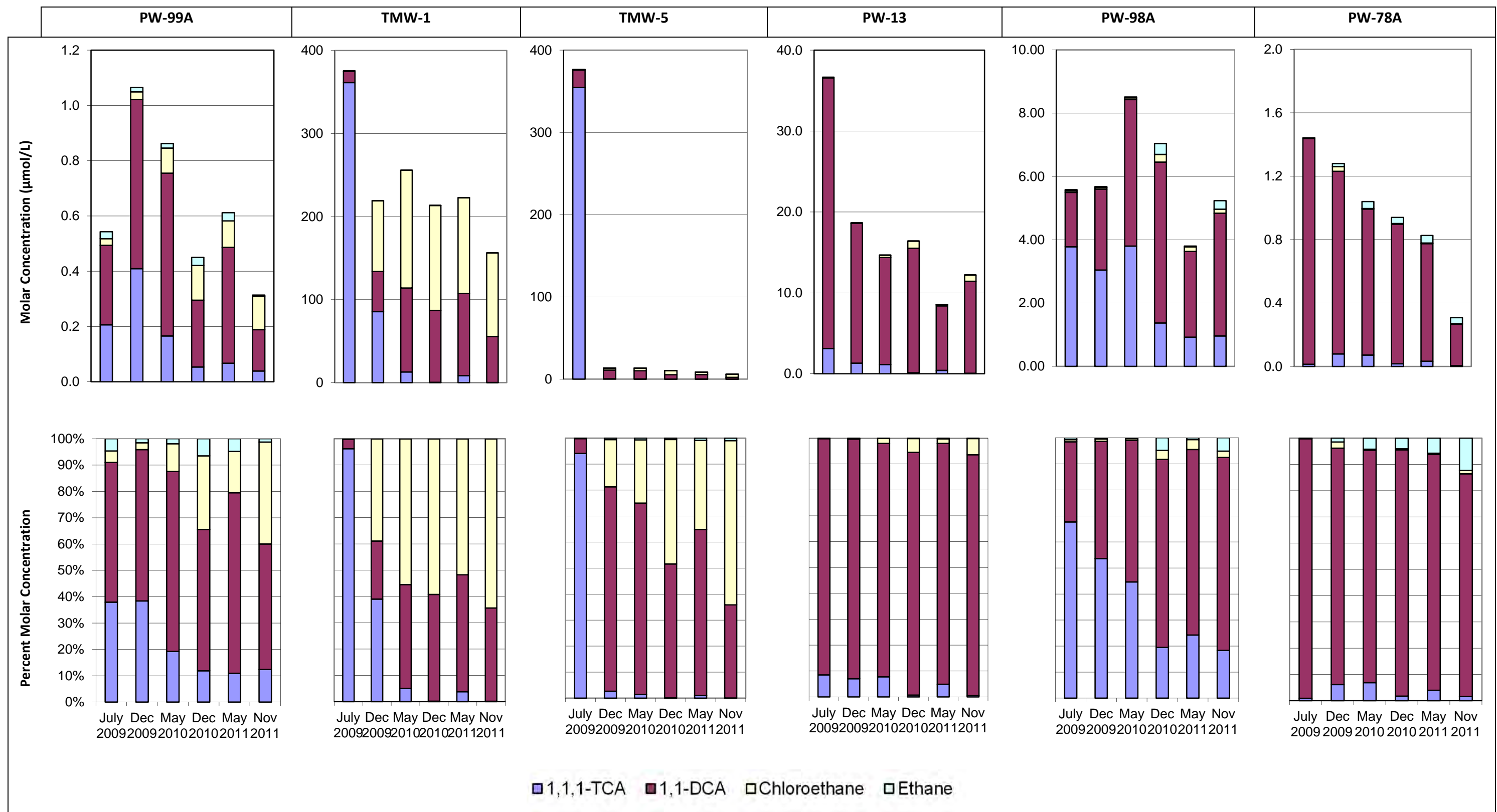
Figure 6-31b. Time Series Charts Showing Chlorinated Ethane Reductive Dechlorination from the ASA Source Area to Down Gradient Wells Wah Chang Five Year Review Report
