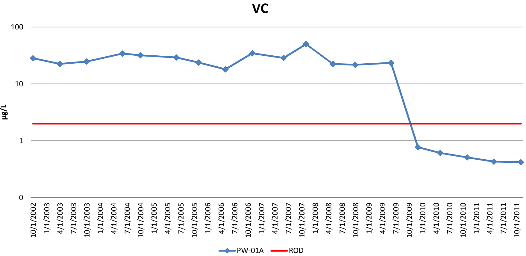
Figure 6-11. VOC Concentrations for Ammonium Sulfate Area Hot Spot Wells in the Fabrication Area
