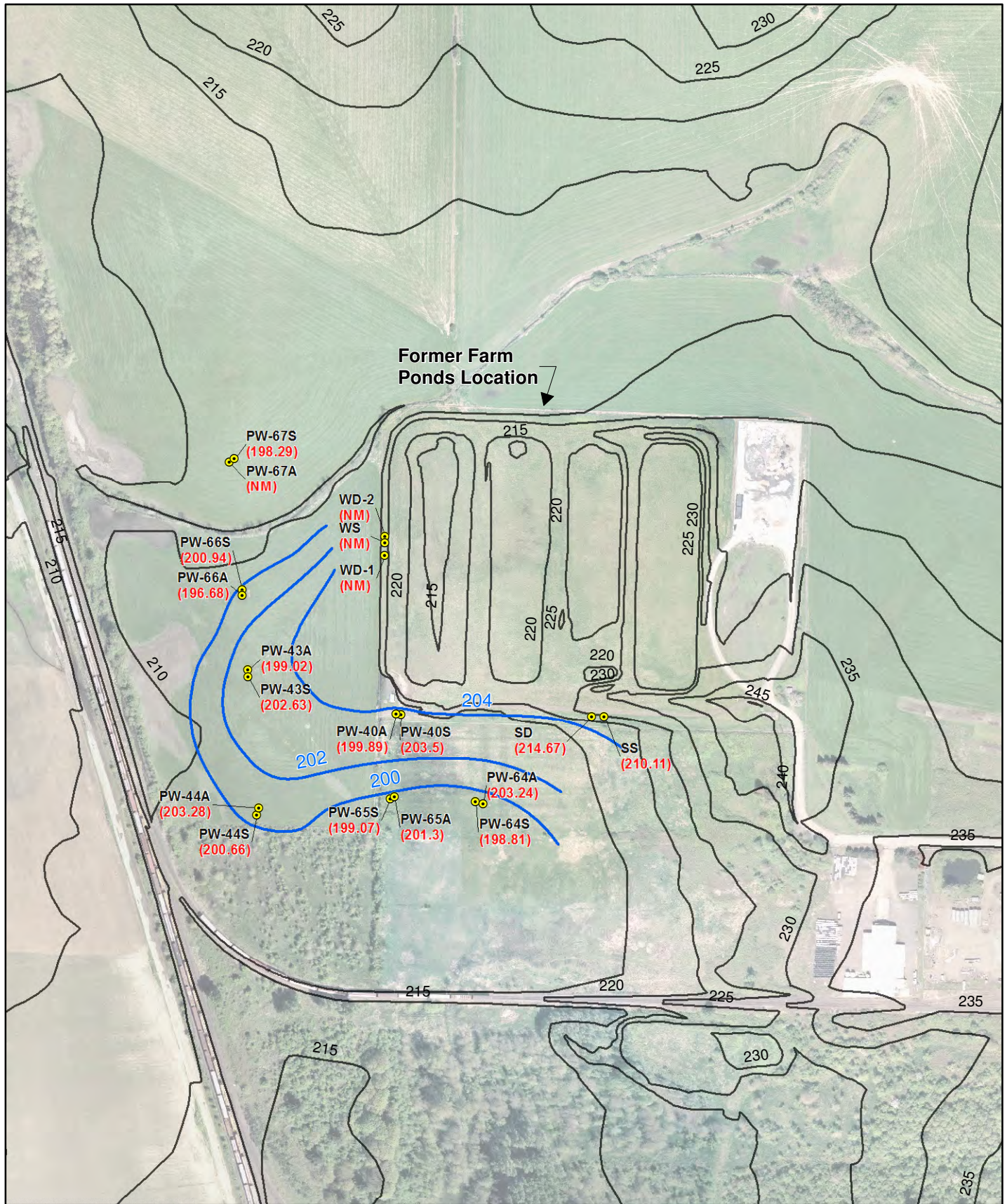
Figure 3-5 Fall 2010 Groundwater Elevation Farm Ponds
