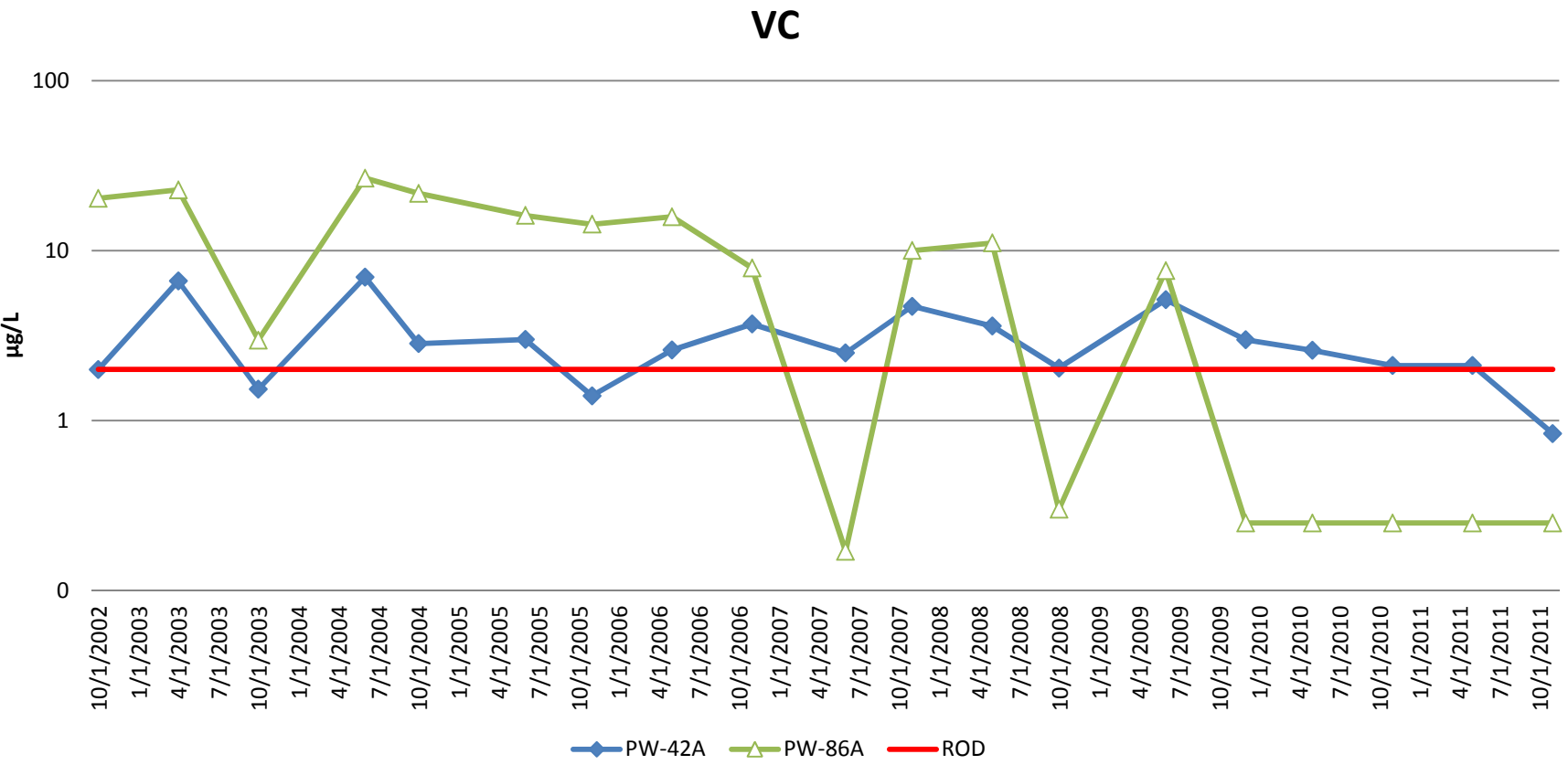
Figure 6-13. VOC Concentrations for Material Recycle Area Hot Spot Wells in the Fabrication Area
