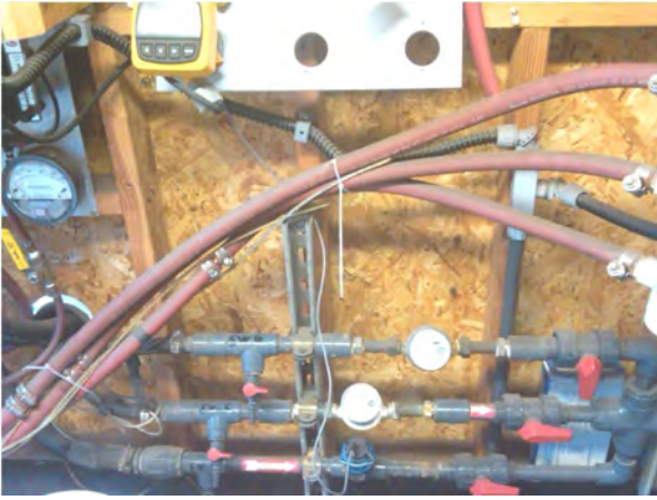
PHOTO – 296 –Treatment system carbon canisters – 2 parallel systems
