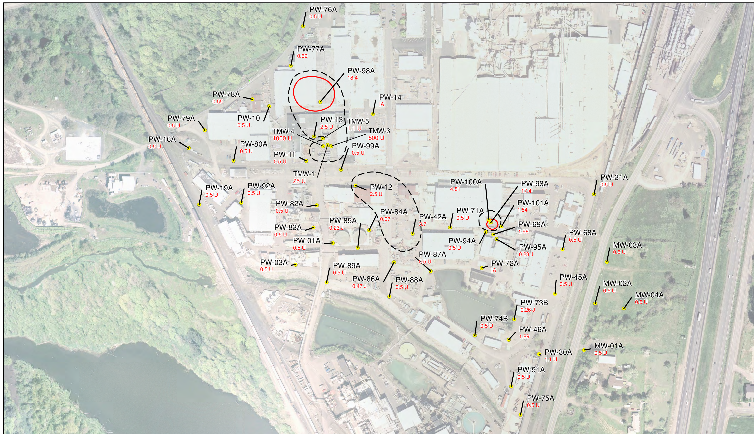
Figure 6-28 TCE Concentrations, Above ROD Fall 2009 and 2011 Fabrication Area
