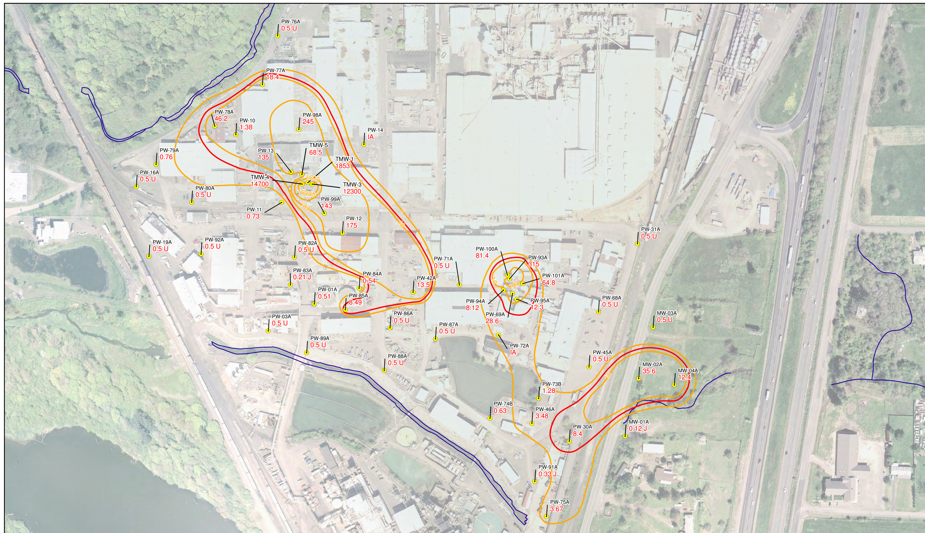
Figure 6-23 DCE Concentrations, Fall 2011 Fabrication Area Teledyne Wah Chang Albany, Oregon
