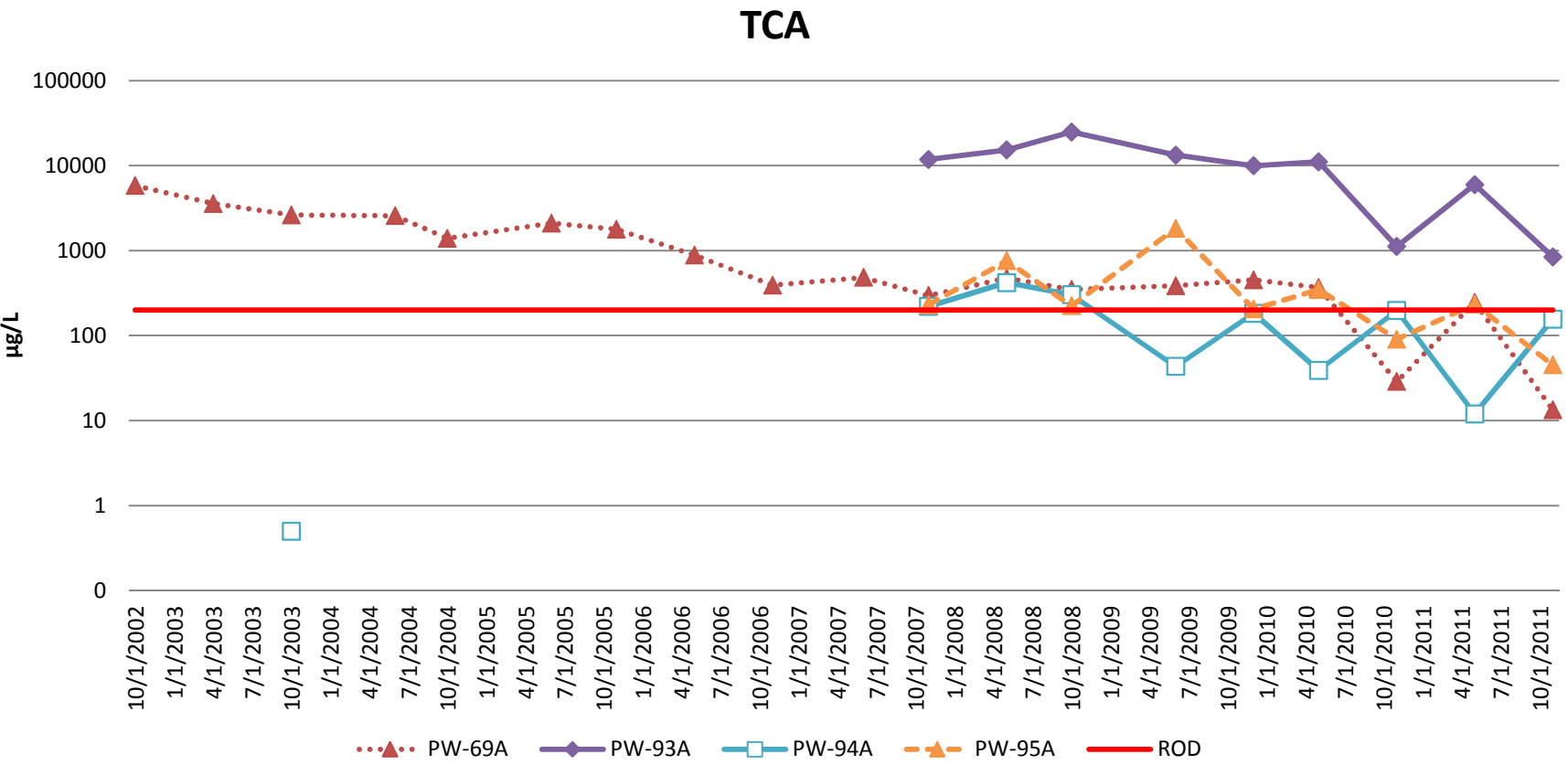
Figure 6-9. VOC Concentrations for Former Crucible Cleaning Area Hot Spot Wells in the Fabrication Area
