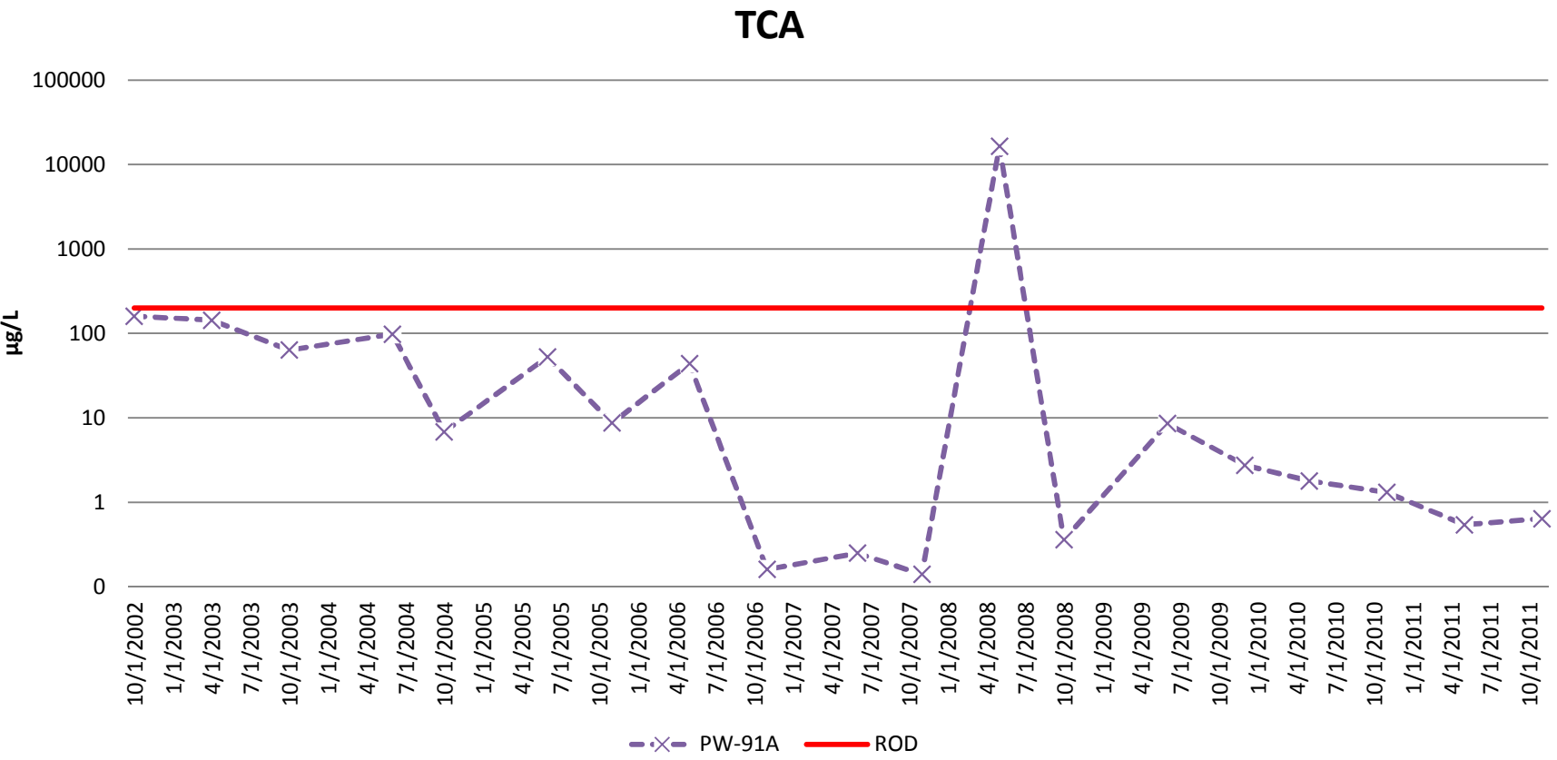
Figure 6-16. VOC Concentrations for Dump Master Area Non-Hot Spot Wells in the Fabrication Area
