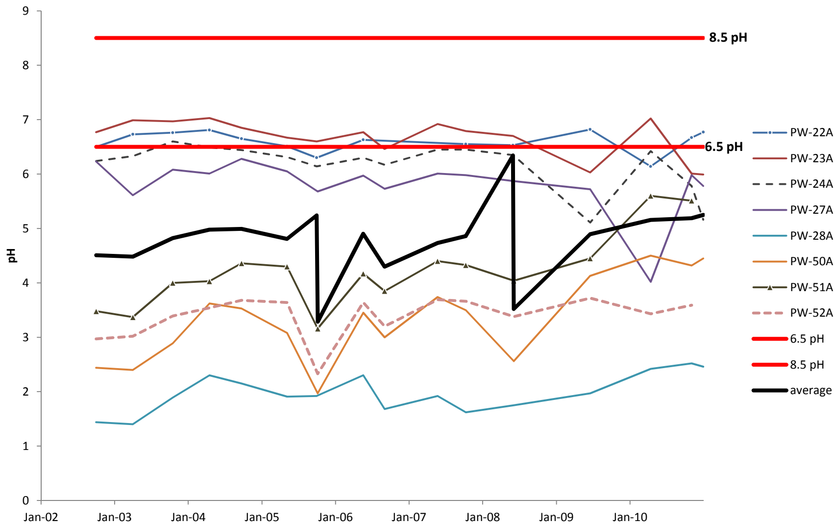
Figure 6-2. FMA pH Level in Groundwater
