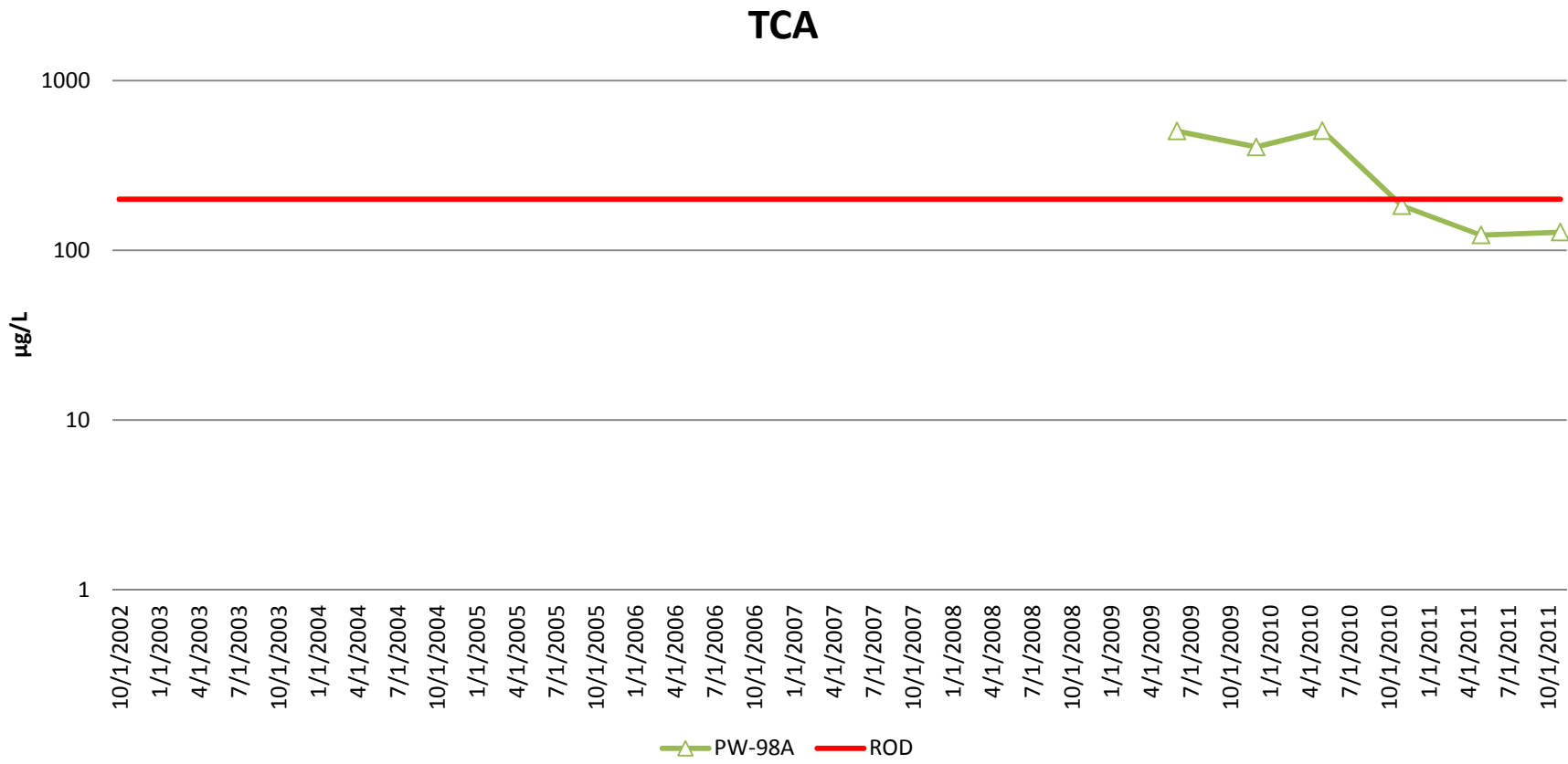
Figure 6-15. VOC Concentrations for Acid Sump Area Non-Hot Spot Wells in the Fabrication Area
