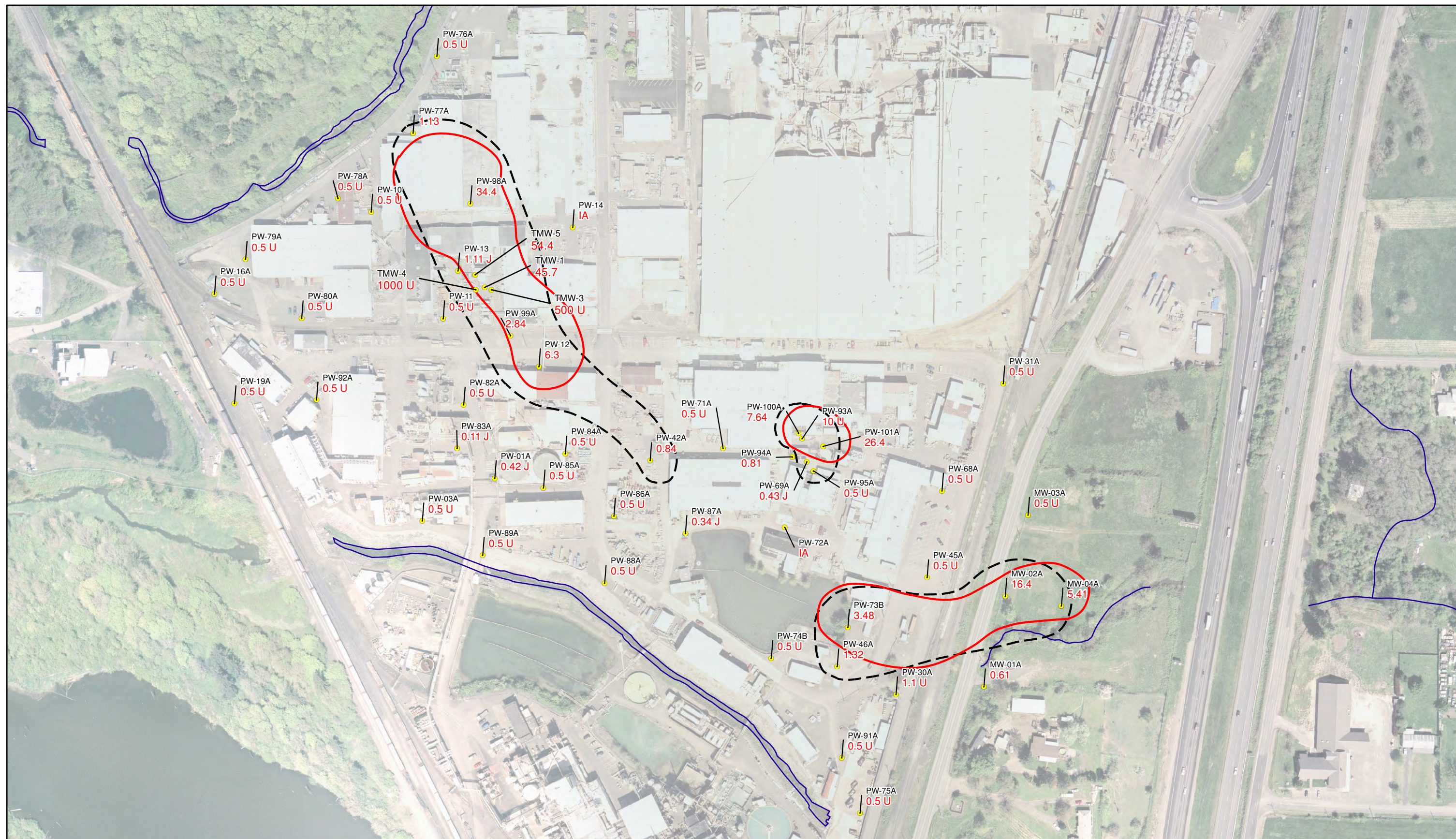
Figure 6-29 VC Concentrations Above ROD Fall 2009 and 2011 Fabrication Area
