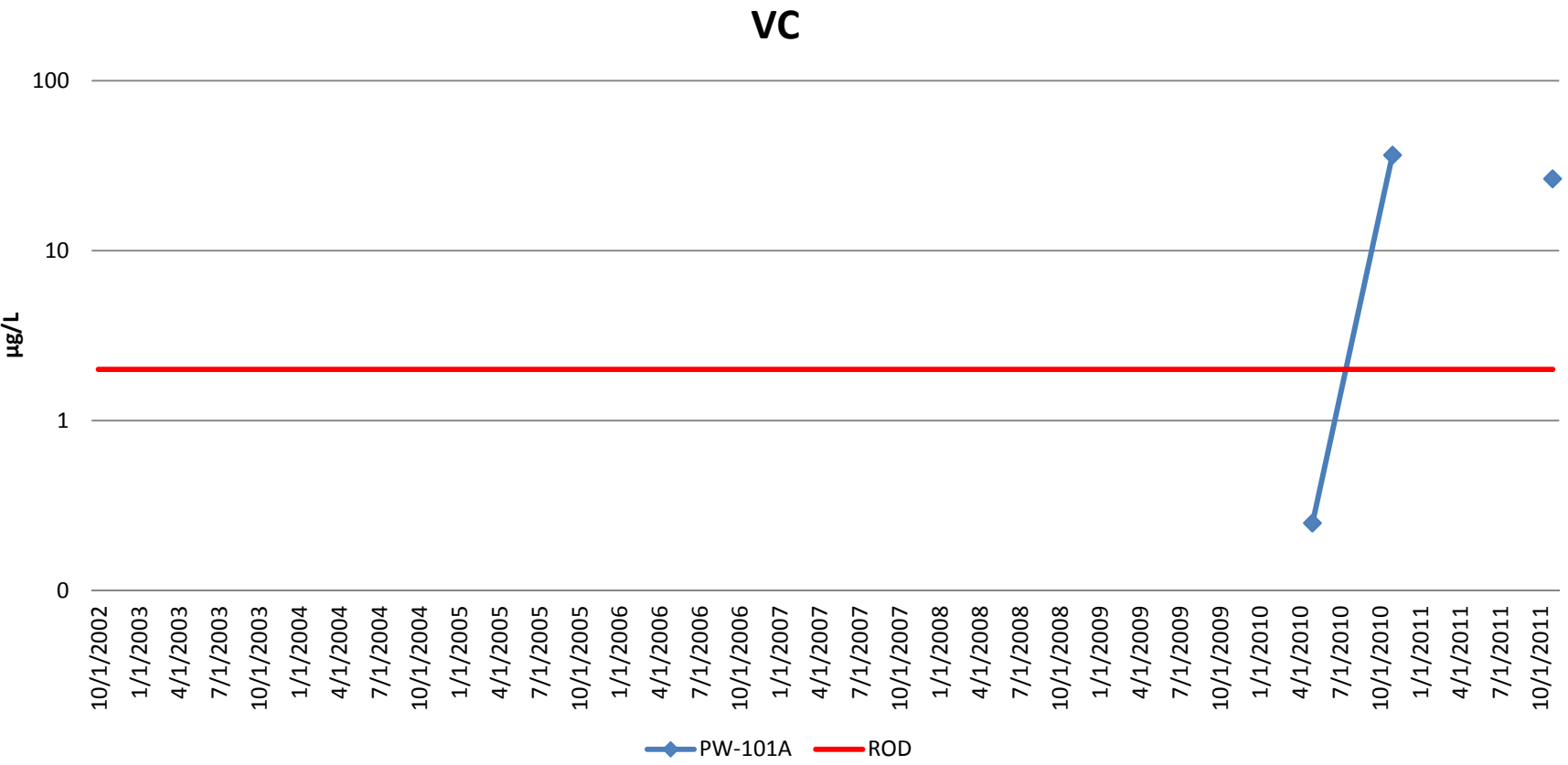
Figure 6-14. VOC Concentrations for Former Crucible Cleaning Area Non-Hot Spot Wells in the Fabrication Area
