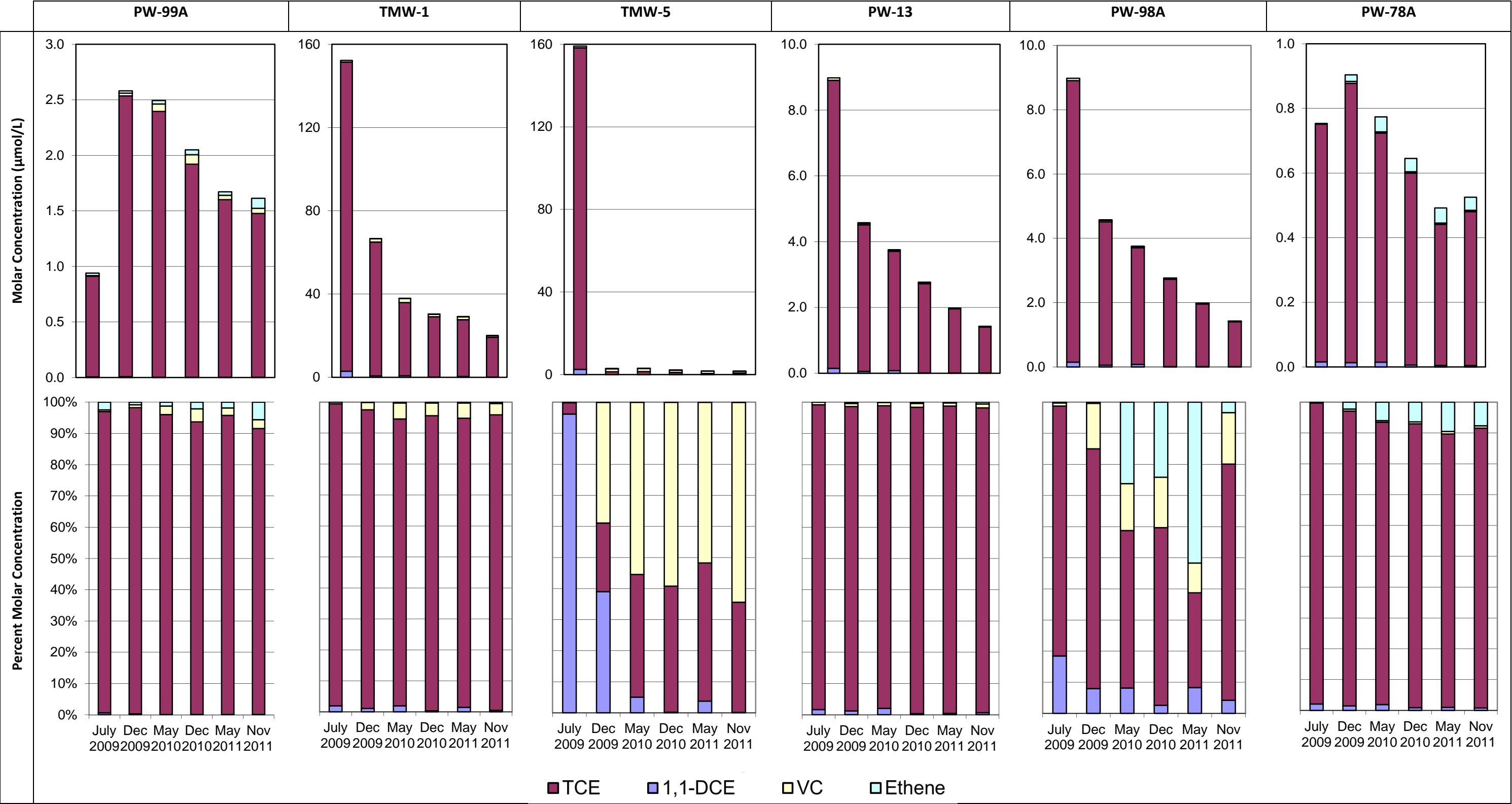
Figure 6-31a. Time Series Charts Showing Chlorinated Ethene Reductive Dechlorination from the ASA Source Area to Down Gradient Wells Wah Chang Five Year Review Report
