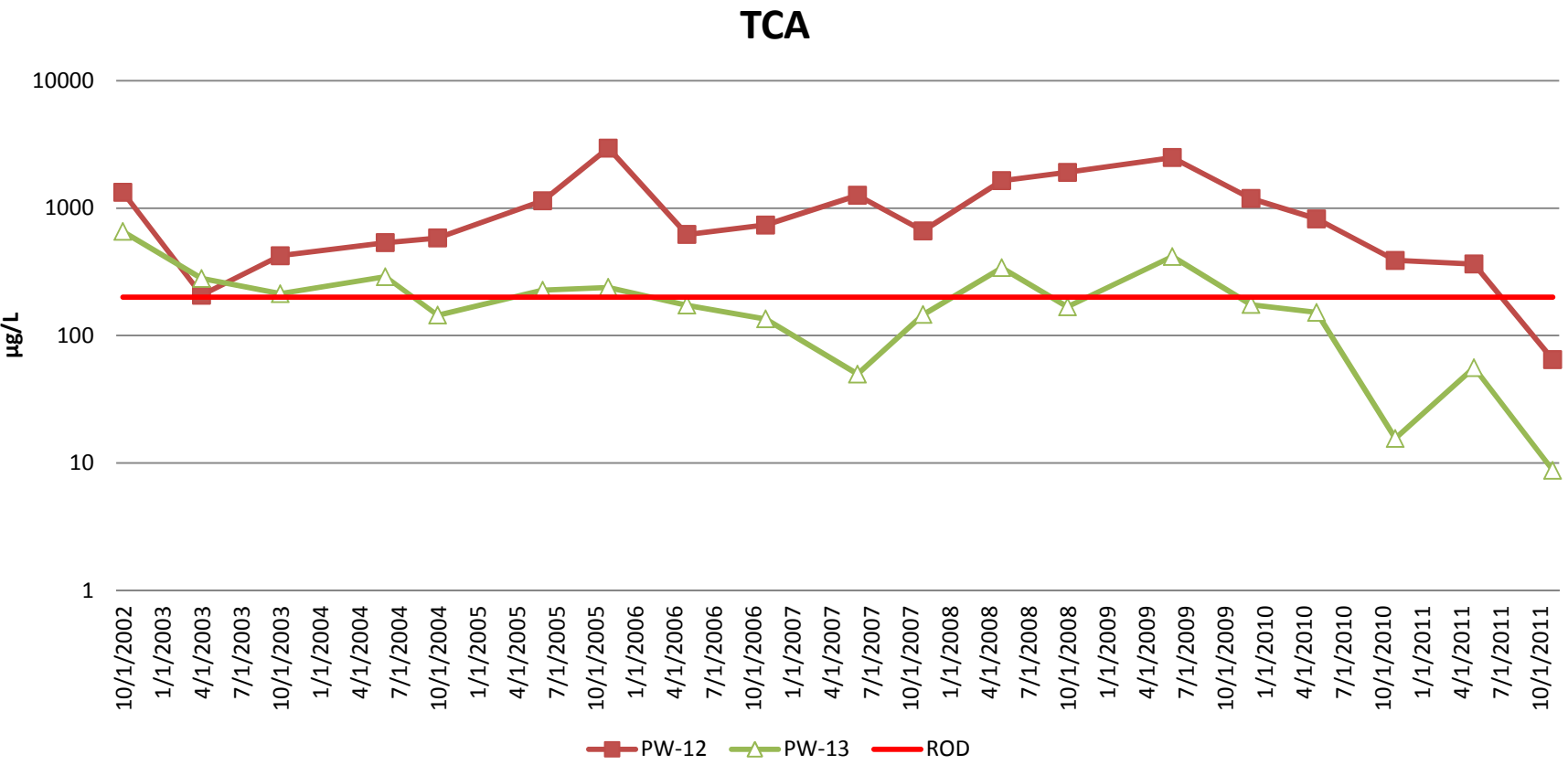
Figure 6-10. VOC Concentrations for Acid Sump Area Hot Spot Wells in the Fabrication Area
