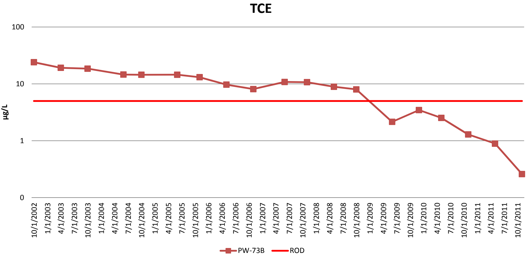
Figure 6-12. VOC Concentrations for Dump Master Area Hot Spot Wells in the Fabrication Area
