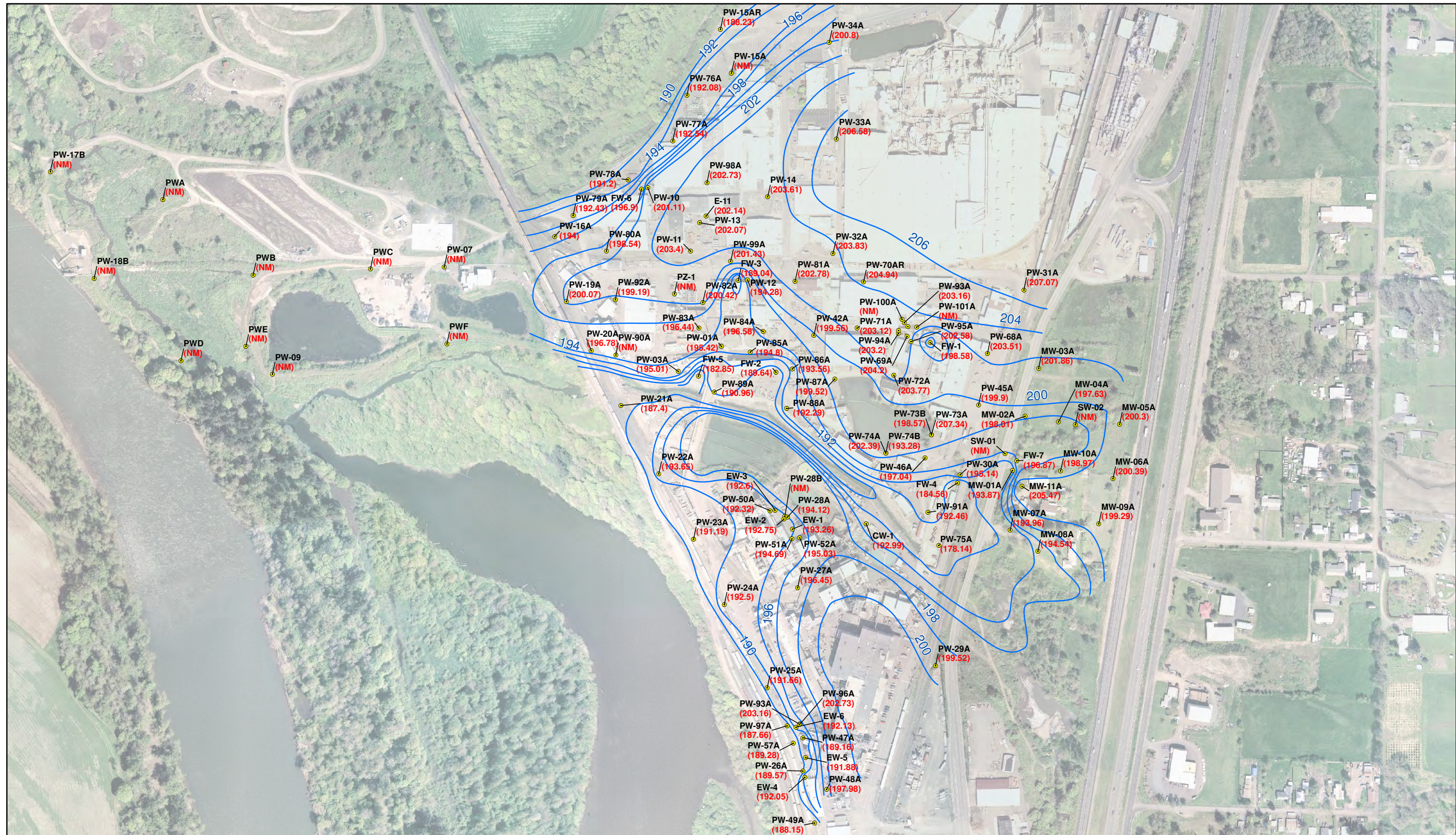
Figure 3-3 Spring 2010 Groundwater Elevation Main Plant
