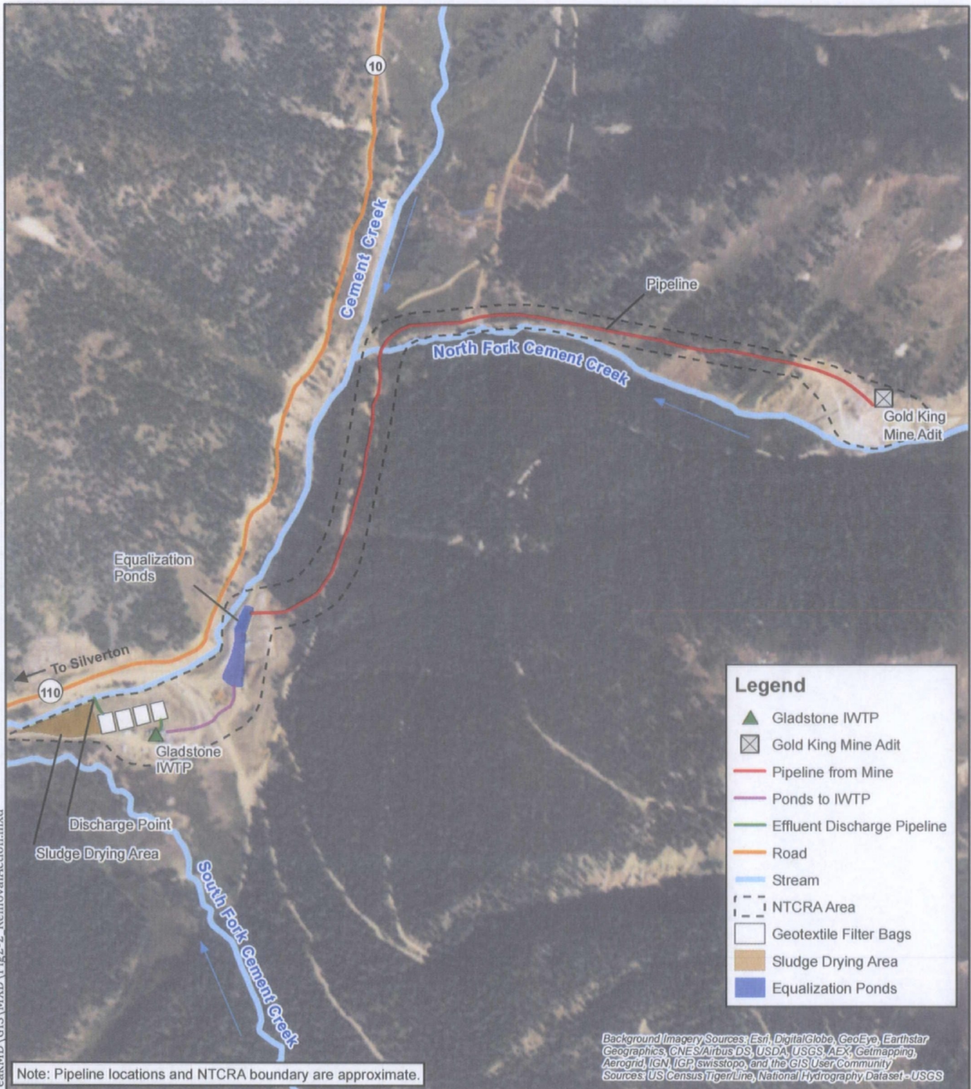
Figure 2 Non-Time-Critical Removal Action Infrastructure Gladstone IWTP AM Bonita Peak Mining District Superfund Site
