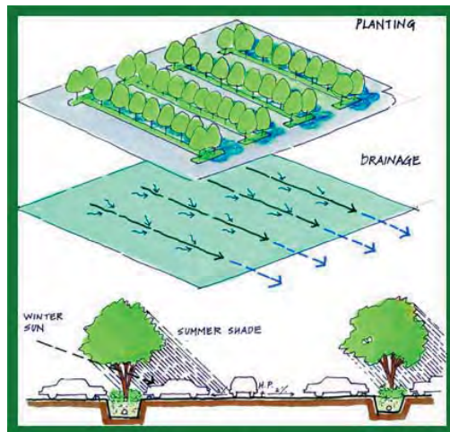
Right and Far Right: Diagram and image of parking facility bioswales, a low-impact design technique developed to help remediate stormwater runoff. Note several key elements of this parking facility bioswale: the cuts in the curb, native plantings, and a center drain. Source: E 2 Inc
