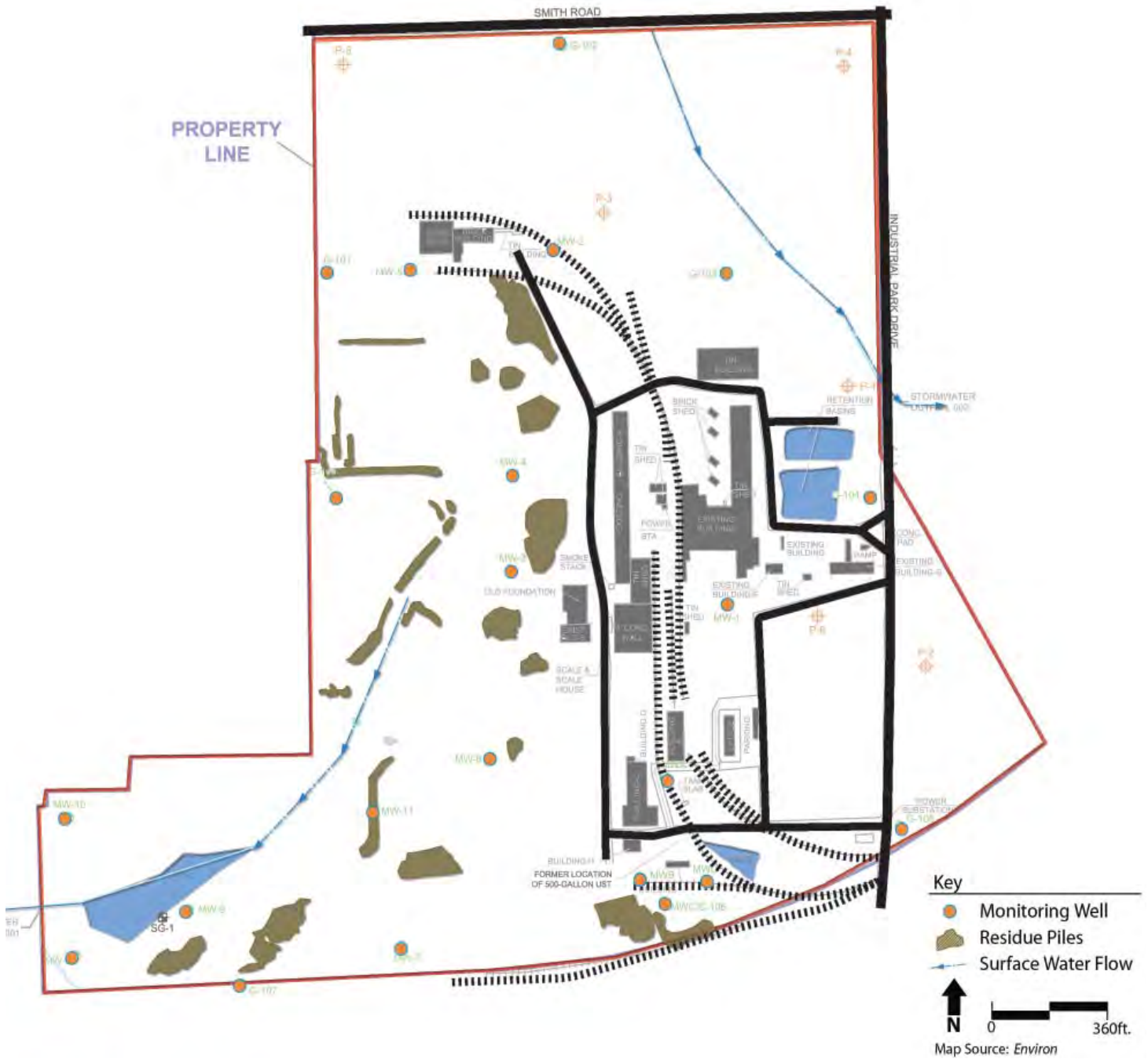
Above: The layout of the Eagle Zinc site as the site exists today. Note the removal of rail spurs and buildings over time, the changes in stream flow and ponds, and the placement of roads and residue piles.
