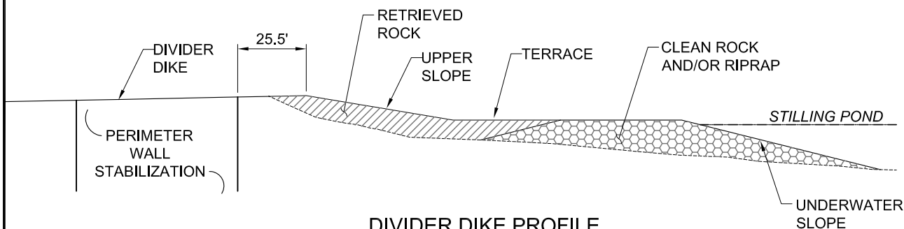
DIVIDER DIKE PROFILE NOT TO SCALE
