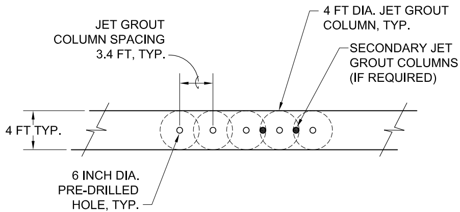
TYPICAL PLAN LAYOUT NOT TO SCALE
