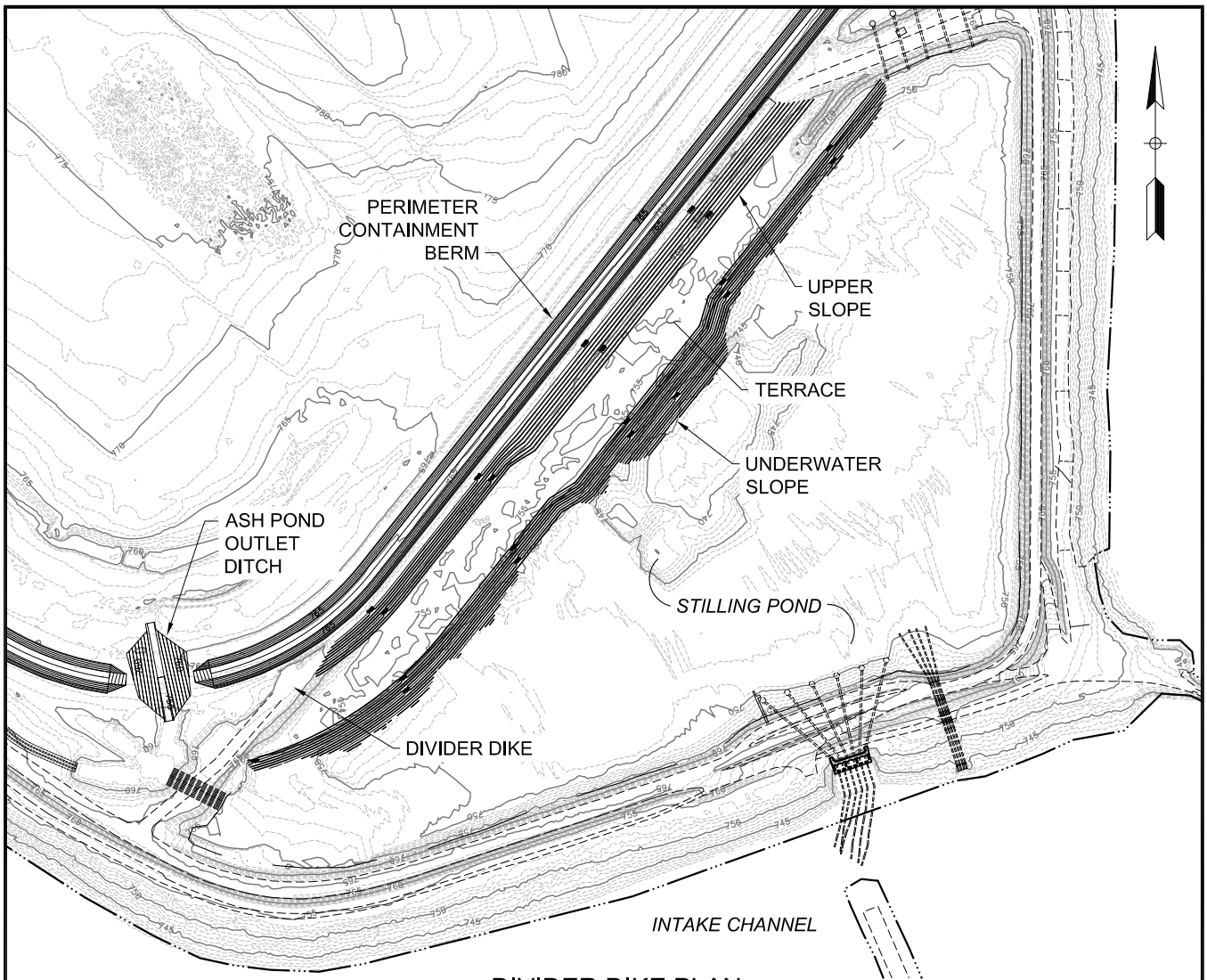
DIVIDER DIKE PLAN 1" = 300'
