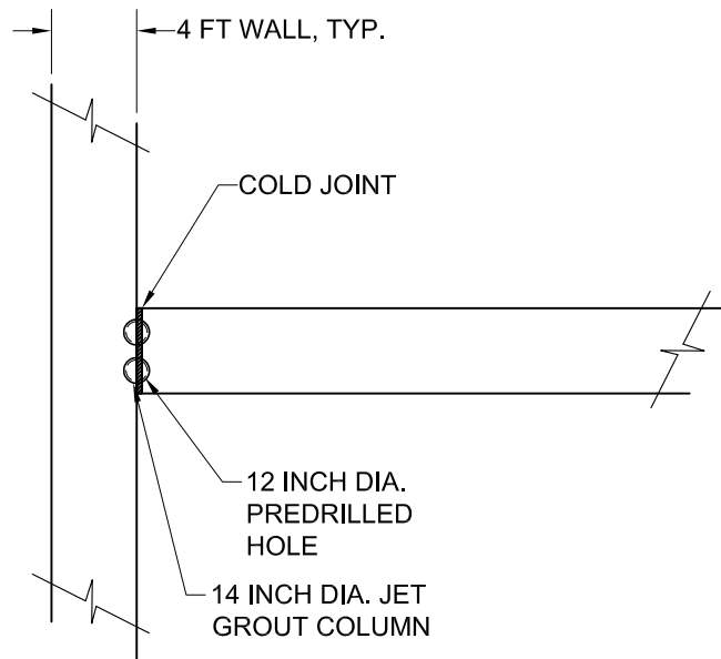
TYPICAL PLAN LAYOUT NOT TO SCALE
