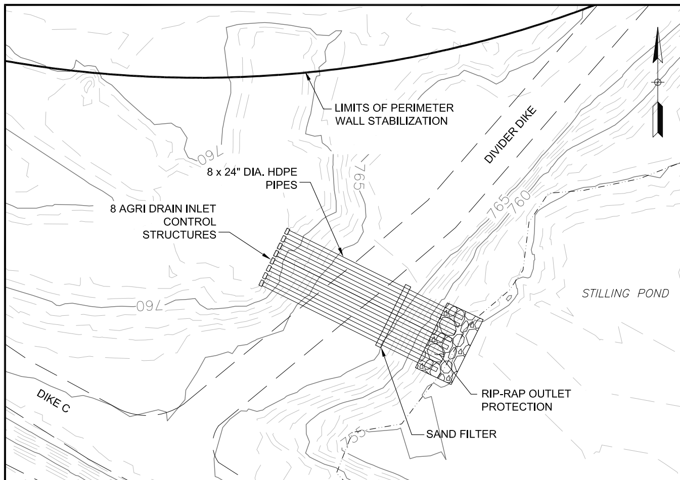
OUTLET STRUCTURE PLAN
