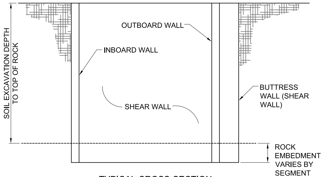
TYPICAL CROSS-SECTION NOT TO SCALE
