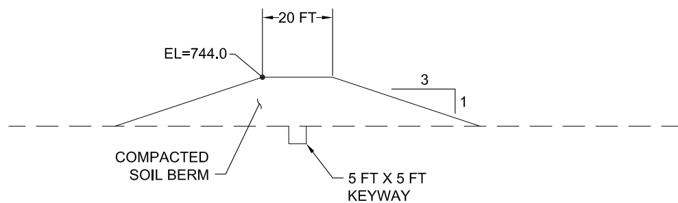
NORTH BERM PROFILE NTS
