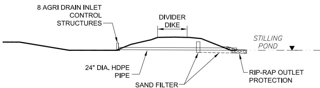
OUTLET STRUCTURE PROFILE
