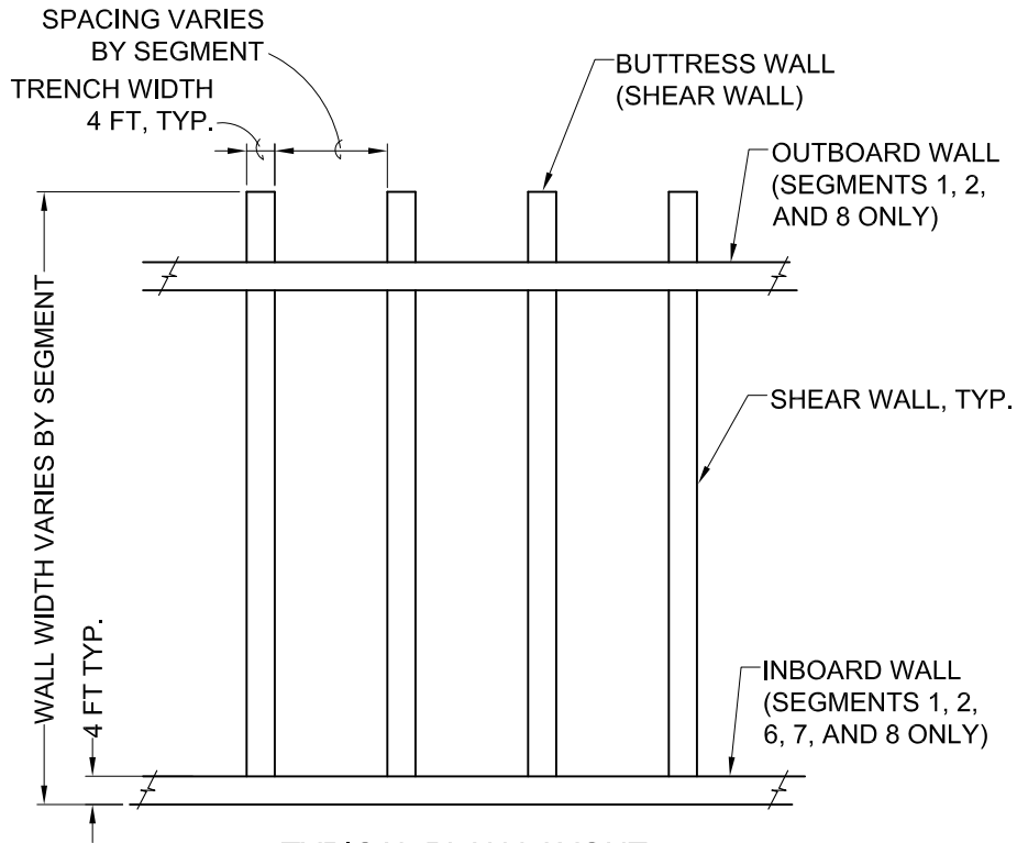
TYPICAL PLAN LAYOUT NOT TO SCALE
