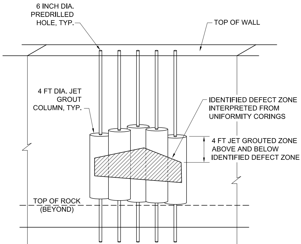
TYPICAL CROSS-SECTION NOT TO SCALE
