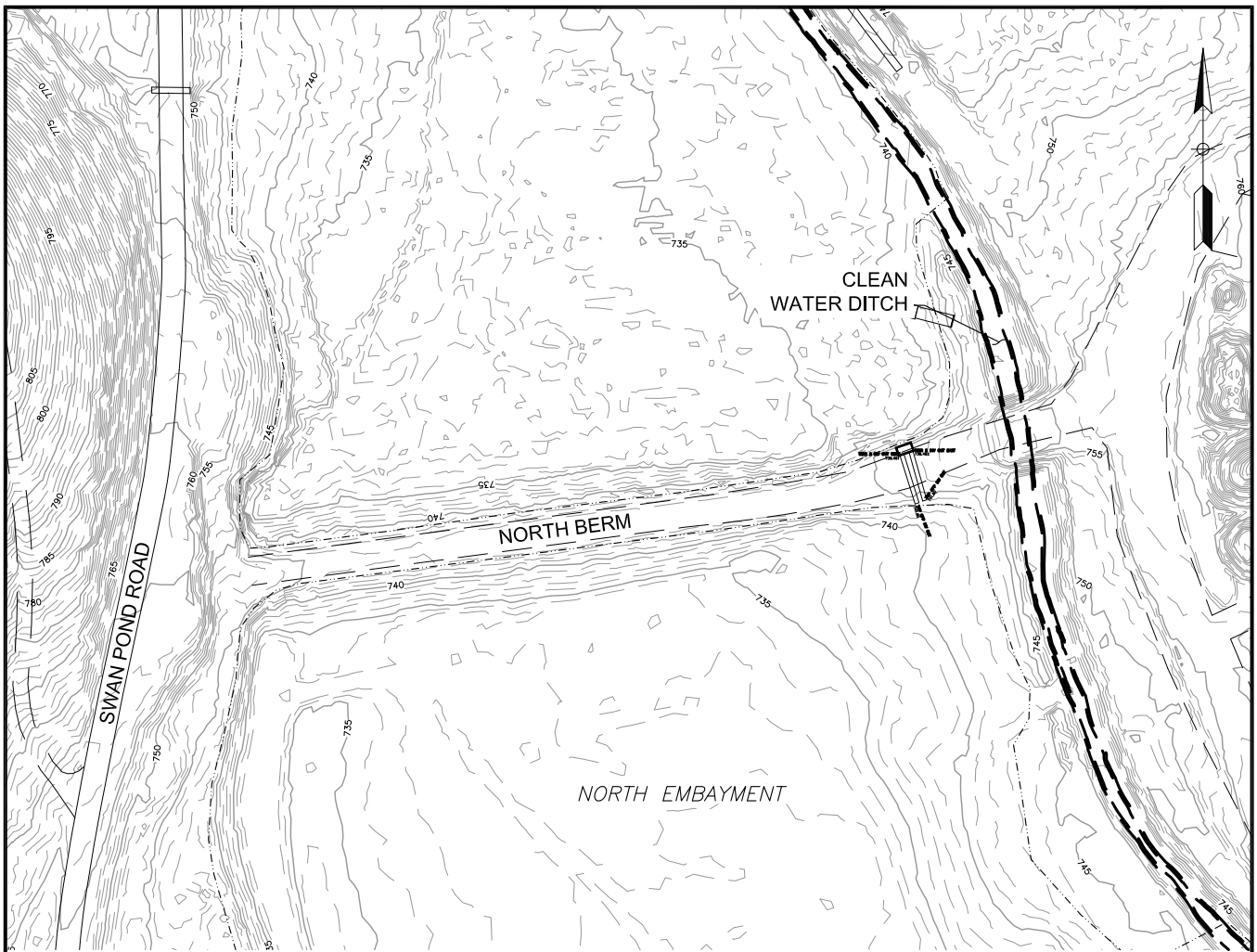
NORTH BERM PLAN
