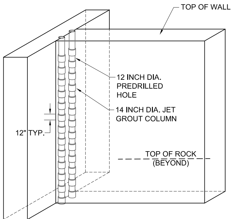
TYPICAL CROSS-SECTION NOT TO SCALE
