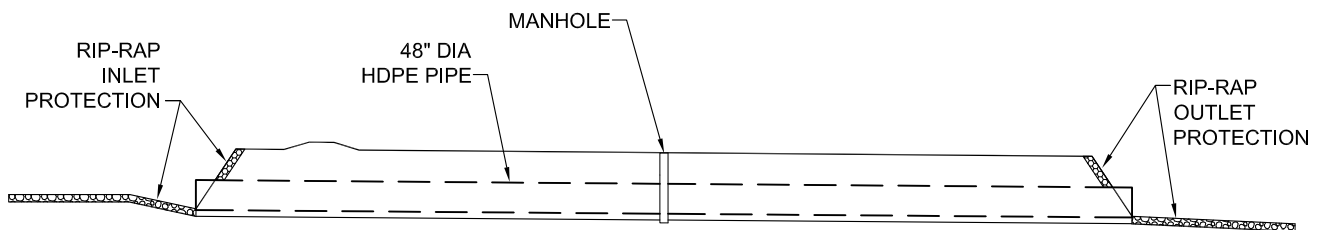
OUTLET STRUCTURE PROFILE
