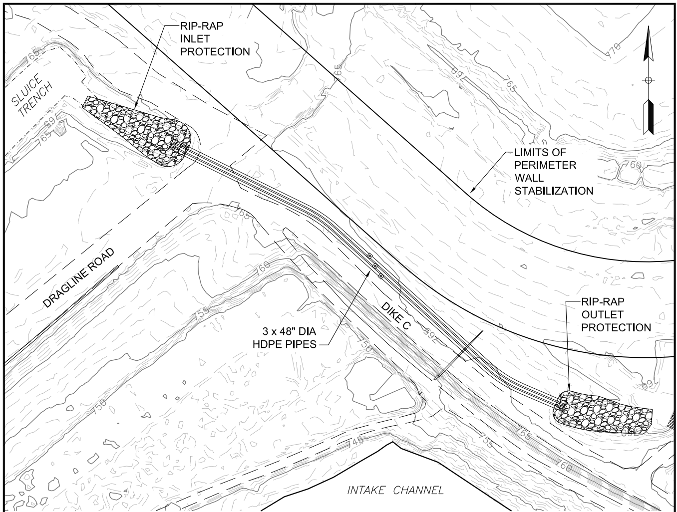
OUTLET STRUCTURE PLAN
